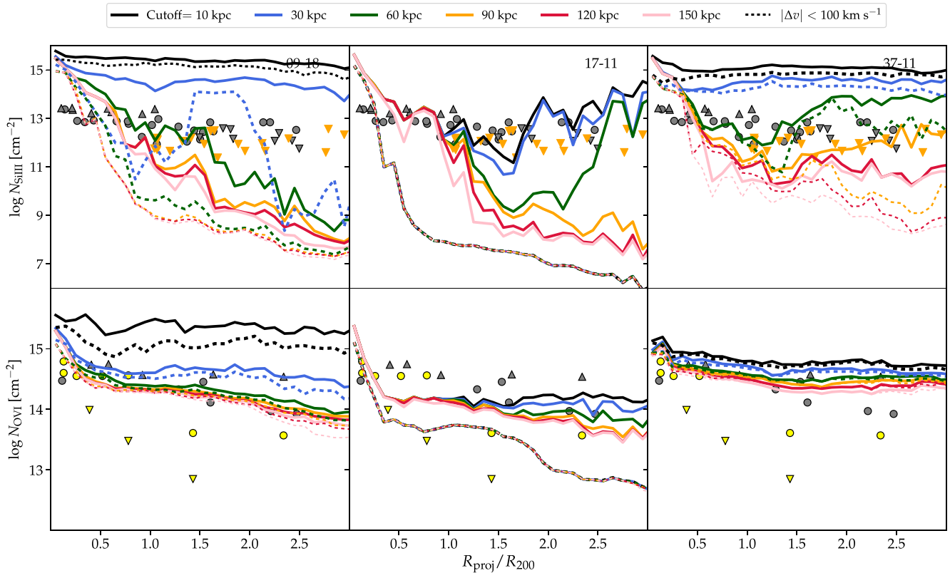
Figure 6. We demonstrate how the gas in the MW’s CGM may influence the observationally derived median column density profiles around M31. We have generated skymaps centred on the MW (instead of the LG, as done in previous figures), where we remove gas lying within a radial cutoff ranging from 10 to 150 kpc from MW (solid lines). For the dashed lines we additionally constrain gas to be within 100 km s −1 of the M31. As in Fig. 5, the data points from Project AMIGA survey (filled grey markers), LC2014 (orange downward markers), and J2015 (filled yellow markers) have been overplotted. Even when only including gas within 100 km s −1 of M31, the Si III profile of 09–18 and 37–11 is increased to \simeq 10^{15} cm −2 by clouds within 10–120 kpc from the MW centre. For 17–11, a velocity selection of gas very well removes gas within 150 kpc of the MW. For O VI, the contamination from the MW’s CGM is also significantly changing the profiles in 09–18 – here gas residing within 150 kpc of the MW may boost the column density by 1.0 dex.
