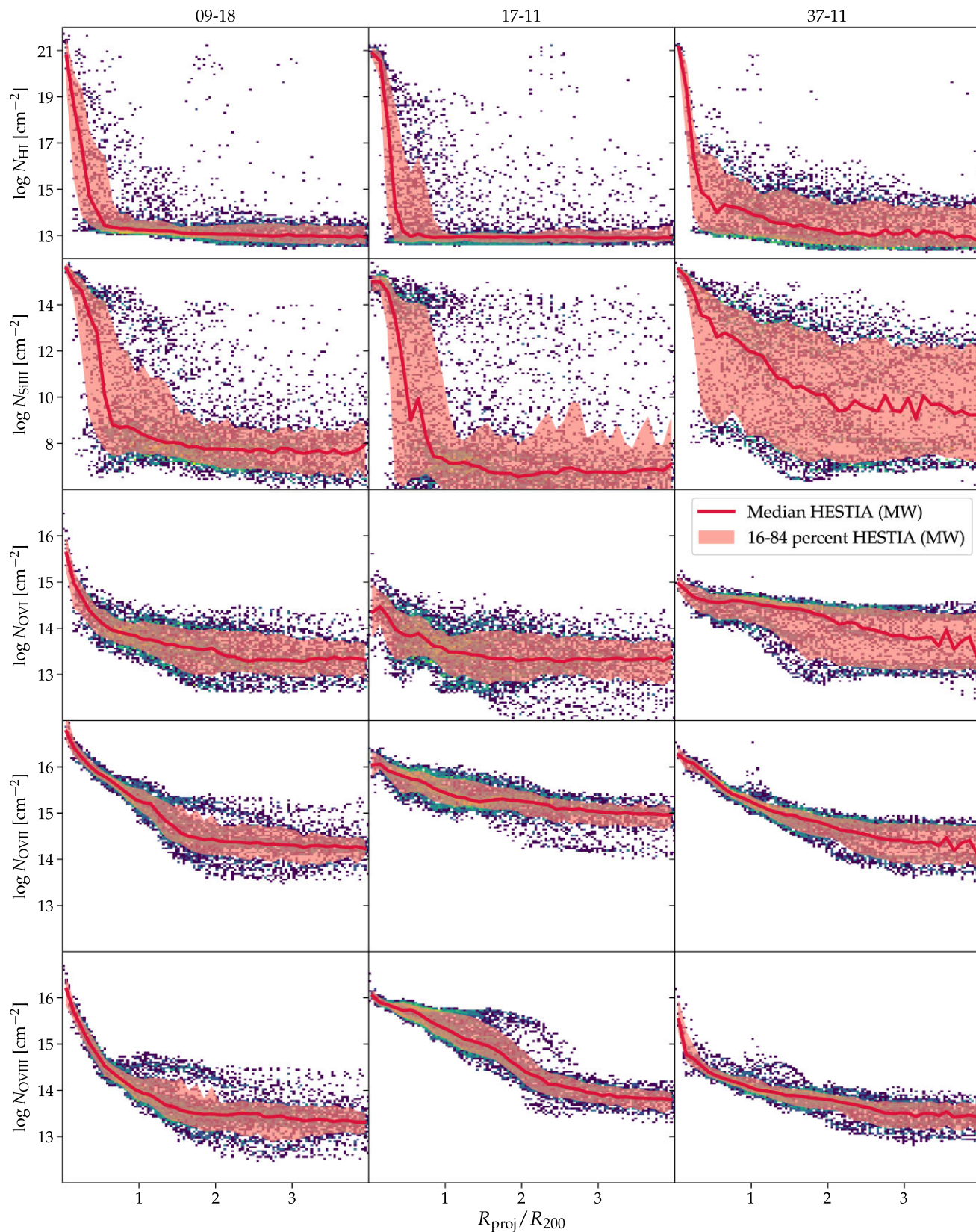
Figure C1. Same as Fig. 4, but for MW. A distinct blob of H I column density absorbers, which can be seen at a distance of \sim 2.0 R_{200} in the H I profile for 09–18, can be correlated with the satellite galaxy numbered 17 in the corresponding skymap (H I skymap for 09–18 in Fig. 1).
