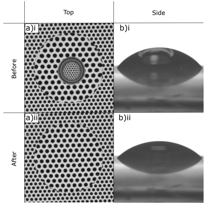
FIG. 6. a) Top and b) side camera images of a droplet-water composite lens i) before and ii) after popping.
