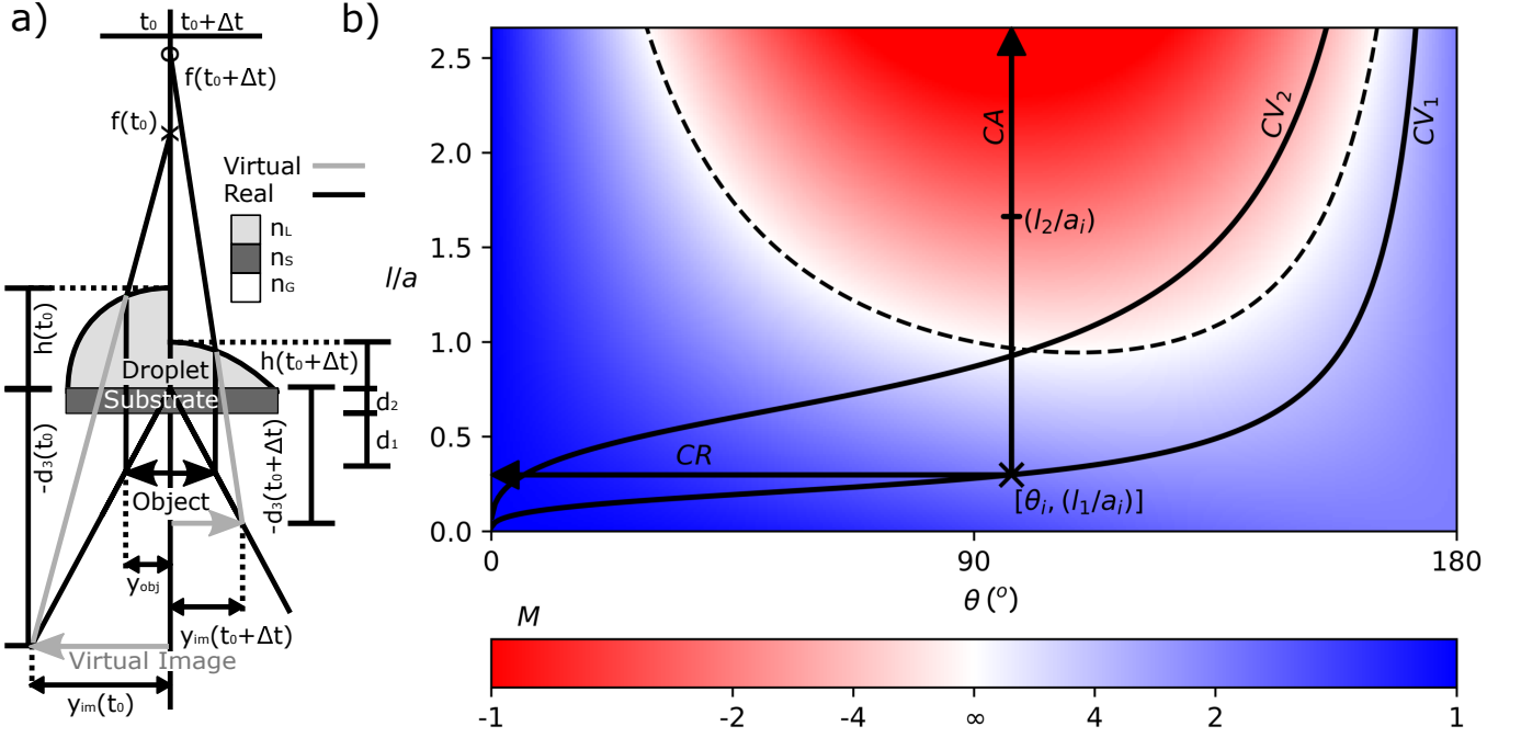
FIG. 1. a) Diagram tracing real (black) and virtual (grey) ray paths from the pattern ( d_1, n_G ), through the substrate ( d_2, n_S ) and droplet ( h, n_L ), to the (virtual) image plane ( d_3 ), for a time t_0 (left) and t_0 + \Delta t (right, of the optical axis). y_{im} is the height of the image formed and f is the focal point of the droplet. b) The magnification M mapped over contact angle ( \theta ) and l/a . Dashed line indicates M = \infty . The black cross at [\theta_i, (l_1/a_i)] indicates the approximate initial position of the droplets in Fig. 2, the vertical and horizontal lines show the evolution of M for CA and CR evaporation respectively. The curved lines indicate the magnifications which can be traversed by an actuated liquid lens of constant volume CV_1 = 10\mu L and CV_2 = 0.1\mu L .
