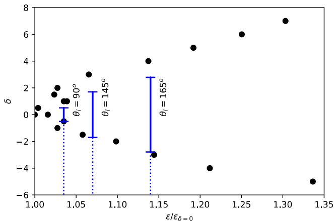
FIG. 3. Variation in normalised dot diameter ( \epsilon/\epsilon_{\delta=0} ) translated a distance \delta from the imaging plane of the CCD camera. The blue bars represent the range of movement in the image plane, for complete evaporation from three initial contact angles ( \theta_i ). The bars are positioned horizontally to encompass the maximum magnification data point within this range when centred vertically at \delta = 0 . The increase in M due to de-focusing is therefore indicated by the dashed lines.
