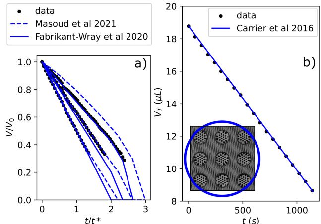
FIG. 4. Experimental data of a 3 \times 3 square compared a) to the predictions of Fabrikant-Wray et al. [16, 23] (solid) and Masoud et al. [17] (dashed) of the normalised volume ( V/V_0 ) against normalised time ( t/t^* ). b) to the radius ( a_s = 5.13\text{mm} ) of a superdrop (blue circle) obtained by fitting the total nine droplet volume ( V_T ) to Carrier et al. [15].
