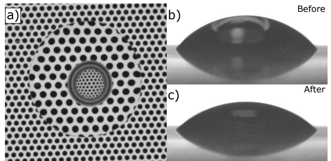
FIG. 5. a) Top camera view of a droplet with an air bubble trapped at its apex imaging a pattern plate beneath. Side camera view of the droplet and bubble b) before and c) after popping.
