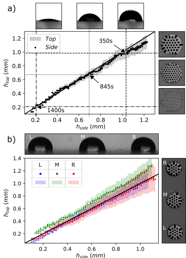
FIG. 2. Height determined by the top camera ( h_{top} ) by substitution of M into Eq. 6 against side camera height ( h_{side} ) for a) an isolated droplet, the surrounding insets show three top and side frames during evaporation. b) three droplet line with the left (L), middle (M) and right (R) colored blue, green and red respectively. The surrounding insets show the first experimental frames from the top and side cameras. The filled regions are the variation in h_{top} due to the uncertainty in the base radius (a).
