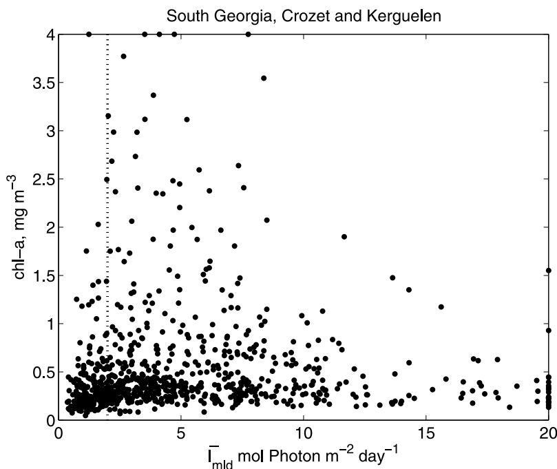
Figure 7. The chl a against \bar{I}_{MLD} for the three HNHC areas, accounting for attenuation caused by chlorophyll and satellite calibration (chl a values are doubled). Note that for plotting reasons, chl a values >4 mg m^{-3} are plotted at 4 mg m^{-3} and irradiance is similarly constrained to 20 mol photons m^{-2} d^{-1} .
