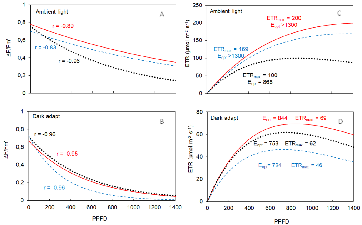
Figure 1. \Delta F_m/F_m' of sago palm seedlings versus irradiances under ambient light condition (A) and dark-adapted condition (B) fitted to an exponential model. ETR versus irradiance under ambient light condition (C) and dark-adapted condition (D) fitted to a Weibull model. Different line colors refer to the time of day when the measurement was performed: morning (red), midday (blue), and afternoon (black). Twelve curves were measured with nine irradiance levels (103 data points) for each time of measurement. PPFD (photon flux density).
