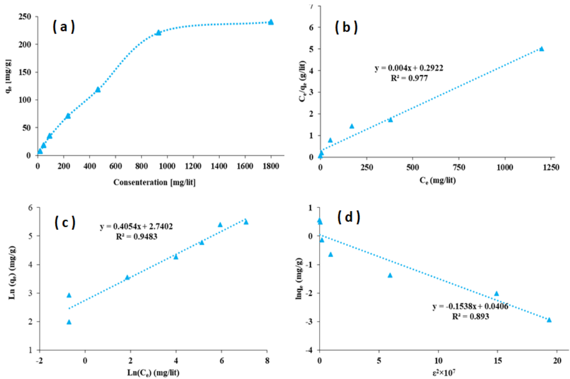
Fig. 8. (a) uptake of Cs(I) at various initial concentrations, (b) straight-line plot of Langmuir model, (c) straight-line plot of Freundlich model, (d) straight-line plots of Dubinin- Radushkevich model
