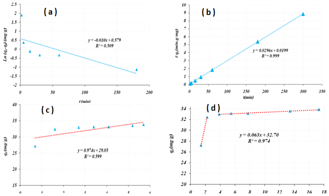
Fig.7. straight-line plots of (a) pseudo-first-order, (b) pseudo-second-order, (c) Elovich, and (d) Morris-Weber kinetic model applied to the uptake of Cs(I) by GO-NiHCFE.
