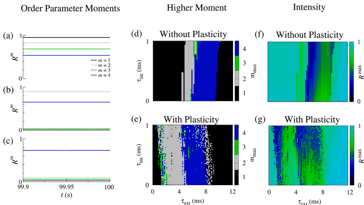
Fig. 5. The panels (a), (b), and (c) show the time evolution of the order parameter moments. We compute the time evolution of the order parameter moments for \tau_{\text{int}} = 0 ms, (a) \tau_{\text{ext}} = 0 ms, (b) \tau_{\text{ext}} = 4 ms, and (c) \tau_{\text{ext}} = 6 ms. The panels (d) and (e) display the symmetric patterns found in the parameter space of \tau_{\text{int}} and \tau_{\text{ext}} without and with plasticity, respectively. The panels (f) and (g) show the highest value of the order parameters moments in the space parameter of \tau_{\text{int}} and \tau_{\text{ext}} for the case without and with synaptic plasticity, respectively.
