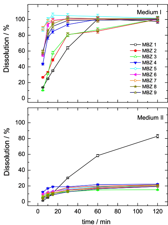
Figure 6. Powder dissolution profiles of the MBZ commercial tablets in 0.1 mol L -1 HCl containing 1% (medium I) and 0% (medium II) of SLS.
