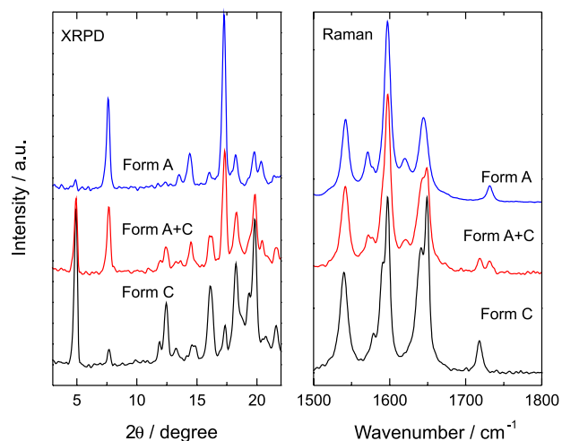
Figure 2. Representative X-ray powder diffraction patterns and Raman spectra of commercial tablets of MBZ.
