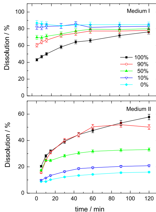
Figure 3. Powder dissolution profiles of MBZ as function of the polymorph C concentration in 0.1 mol L -1 HCl containing 1% (medium I) and 0% (medium II) of SLS.
