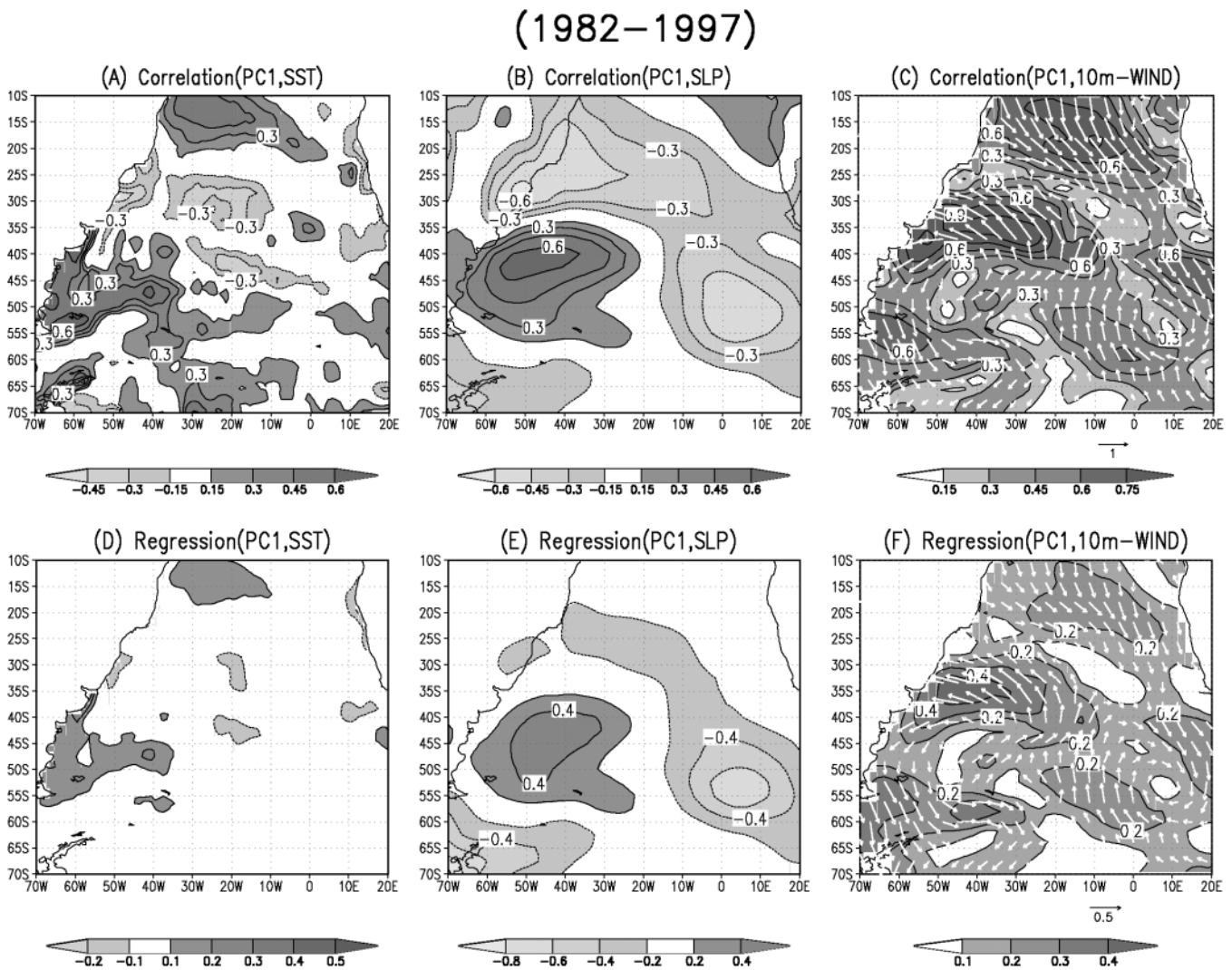
Figure 11. (A) SST, (B) SLP and (C) 10-m wind anomalies correlated upon mode 1 over the South Atlantic ocean (upper panels). Contour interval is 0.15 and zero contour is omitted. (D) SST, (E) SLP and (F) 10-m wind anomalies regressed upon mode 1 over the South Atlantic ocean (lower panels). Contour interval is 0.1^{\circ}\text{C} , 0.2\text{ hPa} and 0.1\text{ m s}^{-1} , respectively. Zero contour is omitted.
