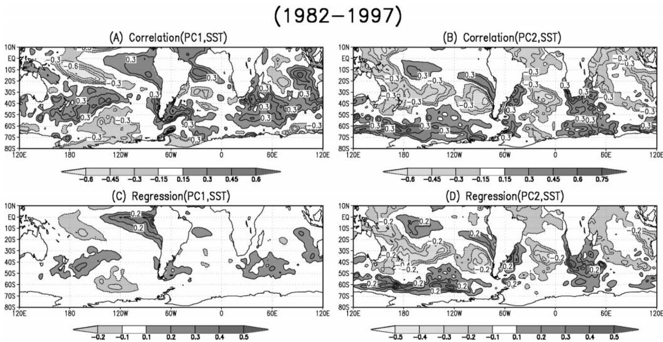
Figure 8. SST anomalies correlated upon the time series of modes (A) 1 and (B) 2. Contour interval is 0.15 and zero contour is omitted. SST anomalies regressed upon modes (C) 1 and (D) 2. Contour interval is 0.1°C and zero contour is omitted.
