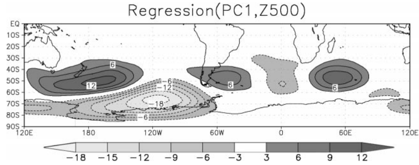
Figure 10. Geopotential heights at 500 hPa (middle troposphere) regressed upon interannual variability mode 1. Contour interval is 3 mgp and zero contour is omitted.
