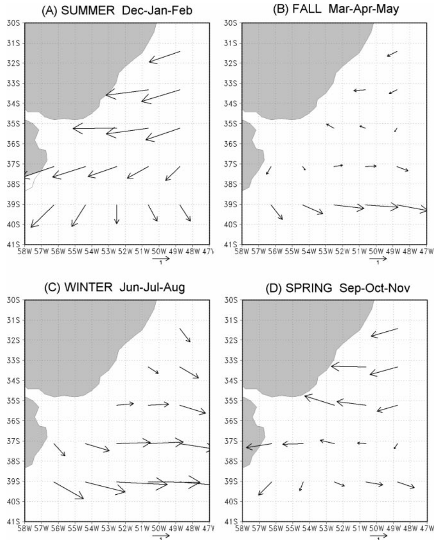
Figure 3. 50-year mean vectors of wind velocity for every season: (A) summer, (B) autumn, (C) winter and (D) spring.
