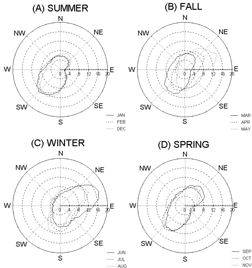
Figure 5. Frequency of occurrence of a given wind direction, computed using the four daily data, by adding the wind speed value every time that it occurs from one of the 72 given direction intervals for every of the year months, for (A) summer, (B) fall, (C) winter and (D) spring.
