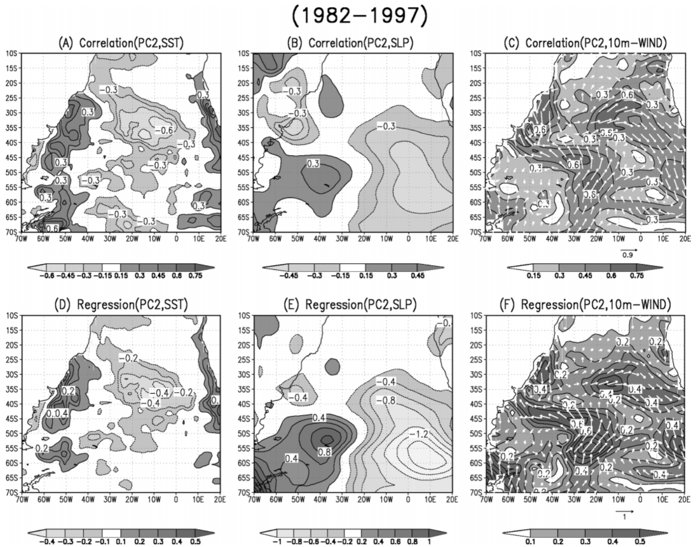
Figure 12. idem figure 11 for mode 2.
