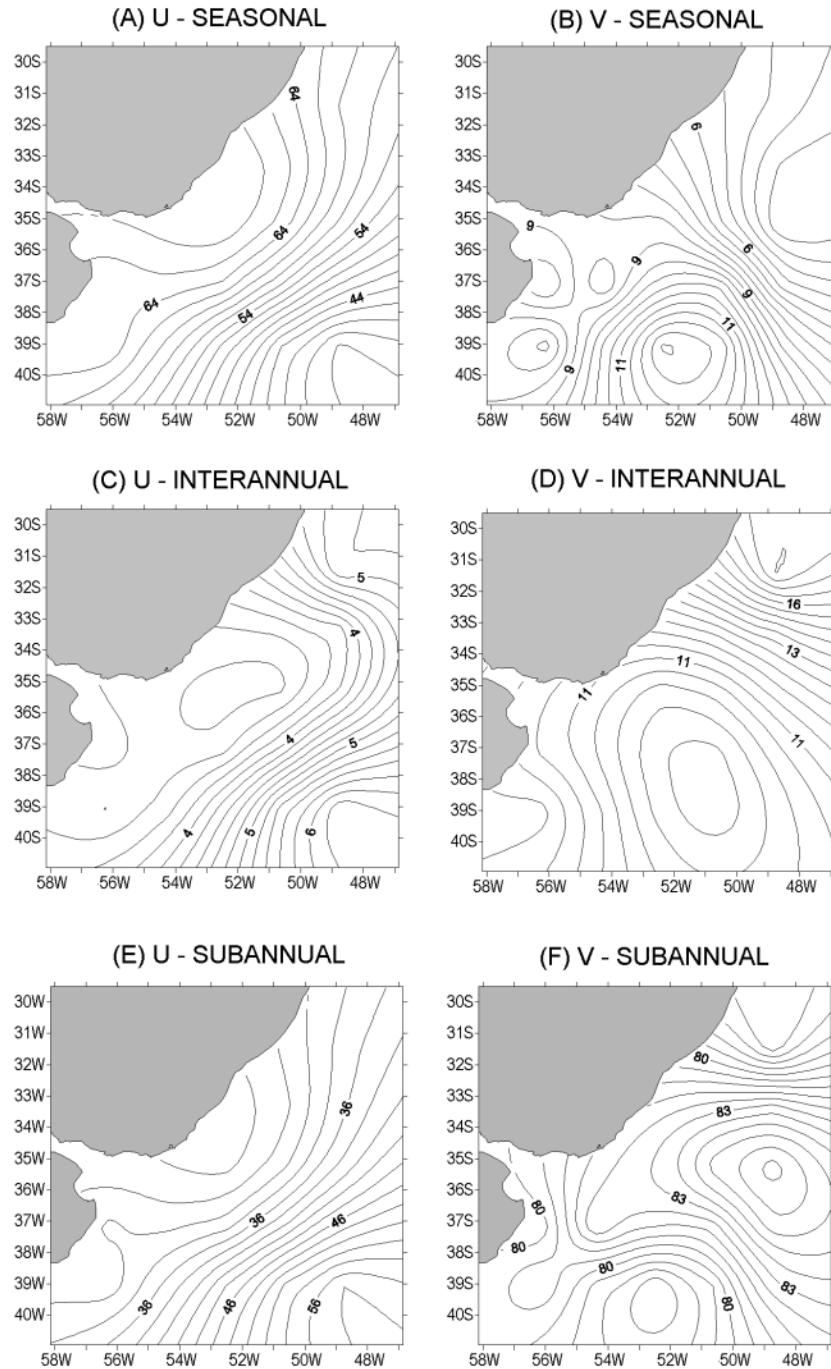
Figure 2. Surface zonal and meridional wind total variance accounted by the (A,B) seasonal, (C,D) interannual and (E,F) sub-annual variability, expressed as percentages of the total variance.
