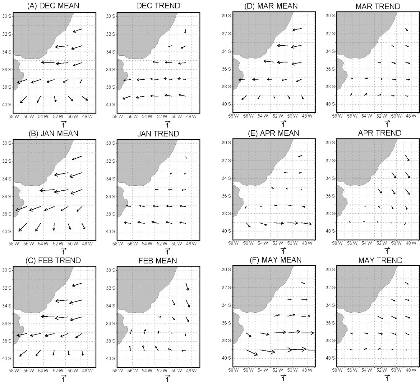
Figure 6. Surface wind climatological monthly means for each calendar month and its respective trend along the 50-year record.
