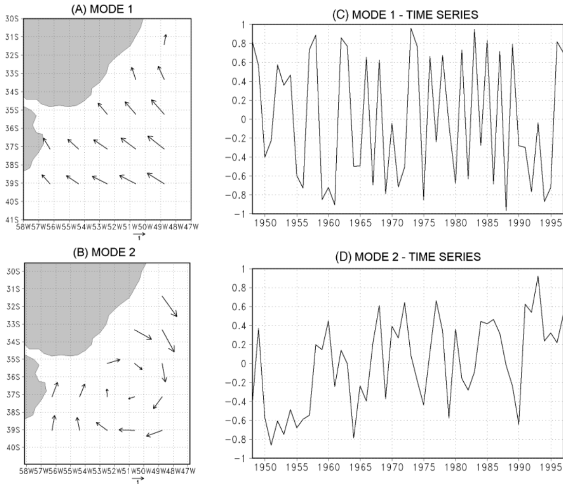
Figure 7. Leading modes of interannual variability for the surface winds obtained from a principal component analysis (t-mode) applied to the annual mean anomalies of the two wind components: (A,B) their spatial patterns and (C,D) the related temporal patterns.
