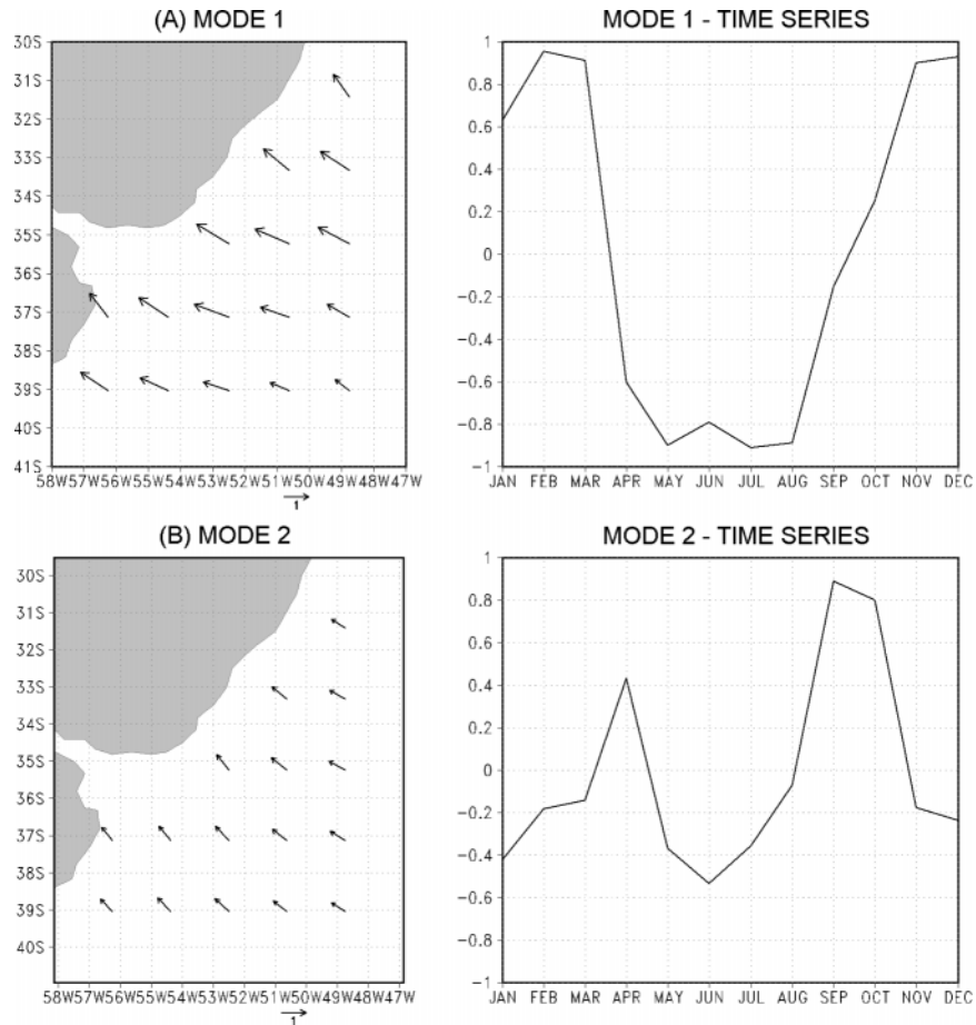
Figure 4. (A,B) Spatial patterns and (C,D) the related time patterns of the two first modes obtained by a principal component analysis on t-mode of surface wind climatological monthly means.
