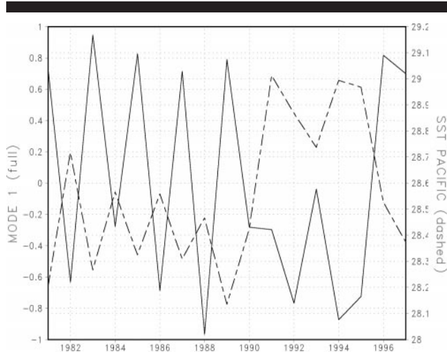
Figure 9. SST variations over the region confined by 10°S–16°S and 170°W–155°W over the western tropical Pacific (dotted line, right axis) and the times series of interannual variability mode 1 (solid line, left axis) during the satellite observational period.
