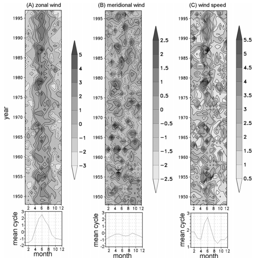
Figure 1. Month vs. year plots of monthly means and climatological seasonal cycles of (A) zonal wind component, (B) meridional wind component and (C) wind speed, for the 1948–1997 period.
