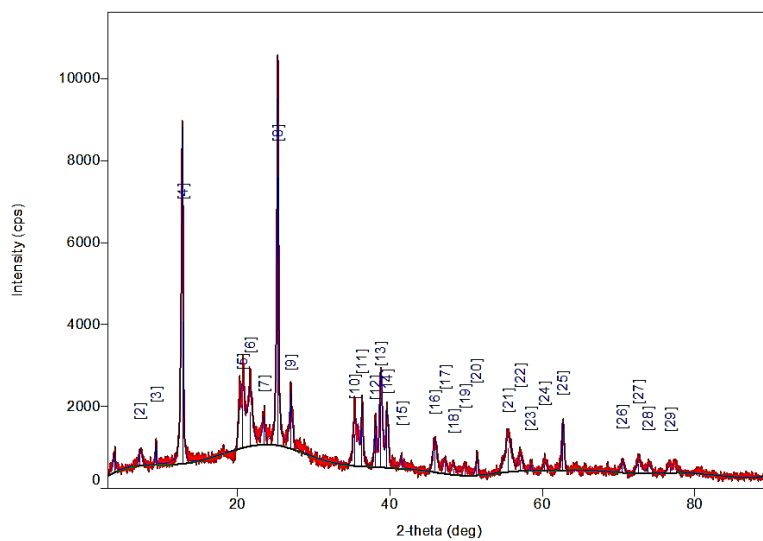
Figure 1. XRD spectrum of natural Kaolin from Bangka
