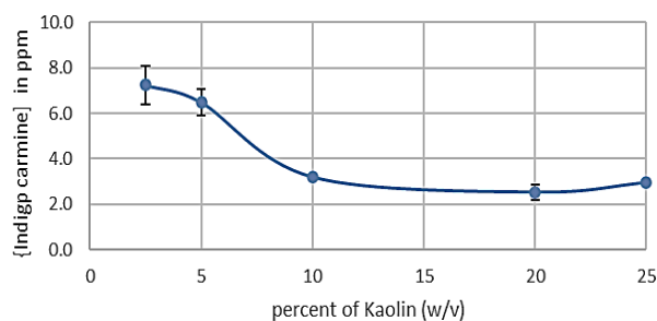
Figure 5. The kaolin dosage influences indigo carmine adsorption.
