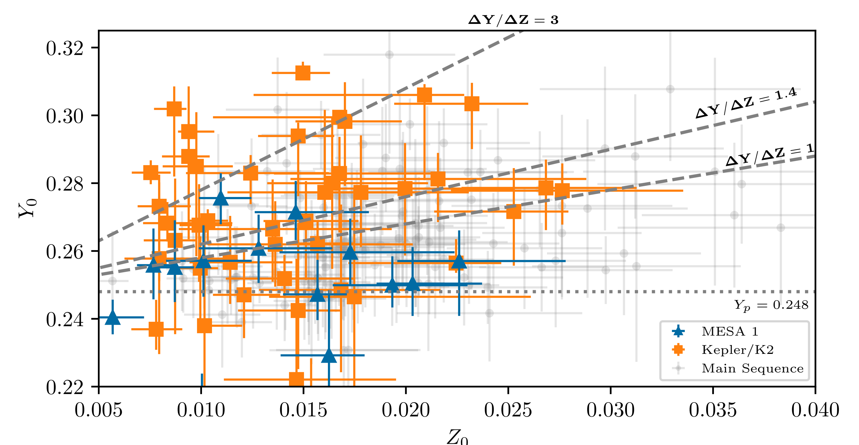
Figure 5: Inferred quantities from stellar modelling; literature values from main-sequence Kepler solar-like oscillators are also included in this figure
