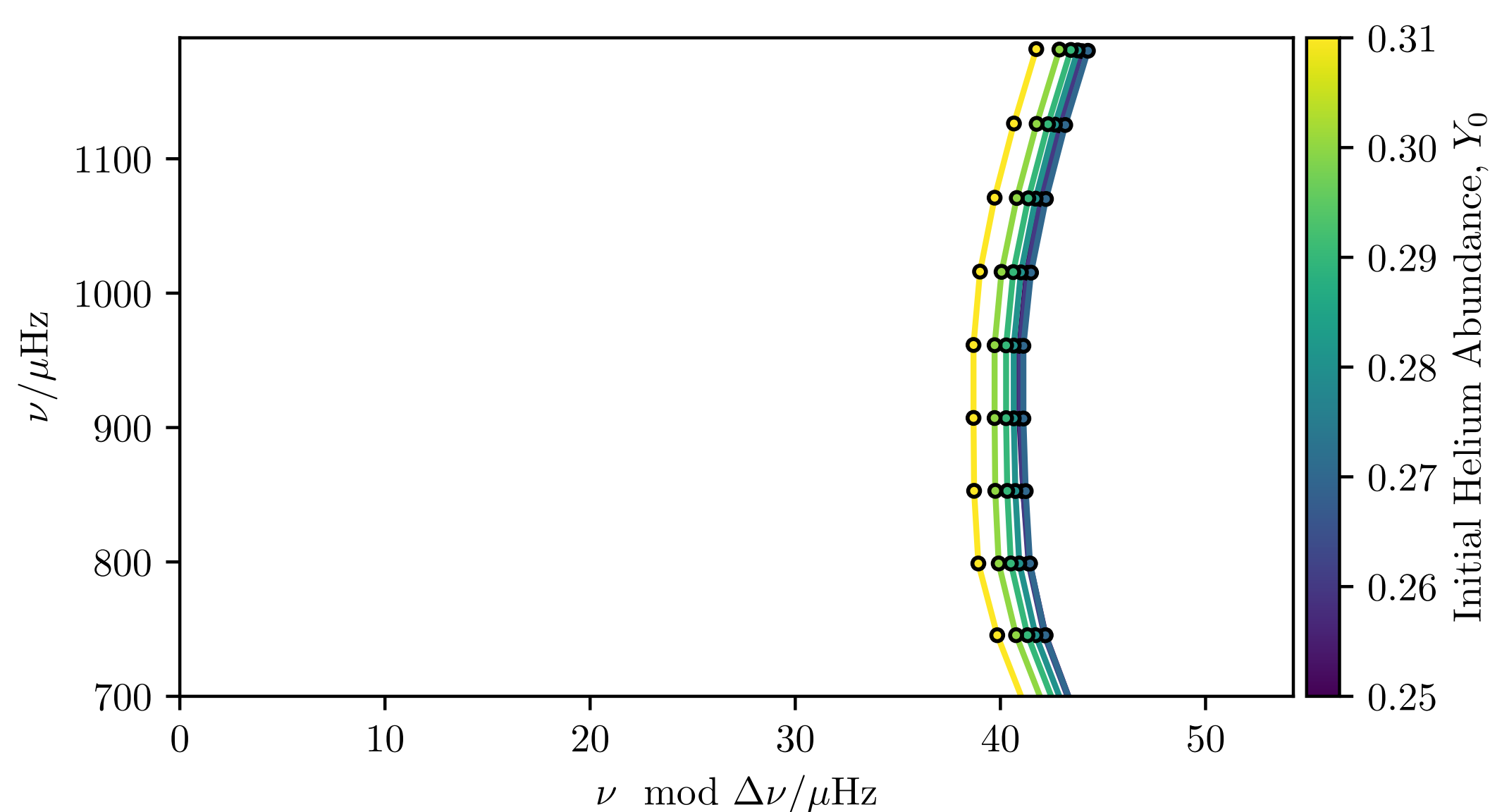
Figure 2: Echelle diagrams of notional pure p-modes for subgiant stellar models
