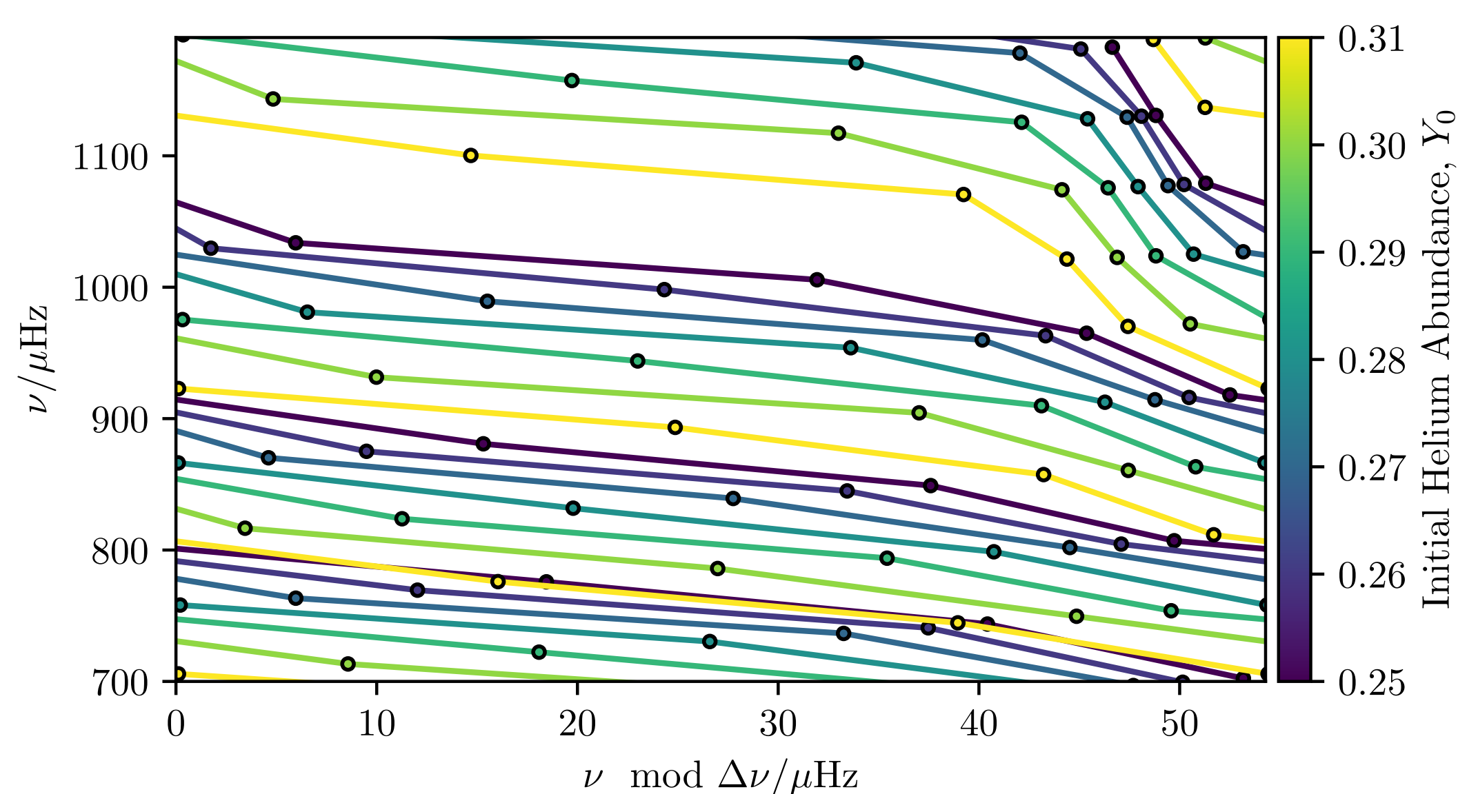
Figure 3: Echelle diagrams of dipole mixed modes for the same stellar models
