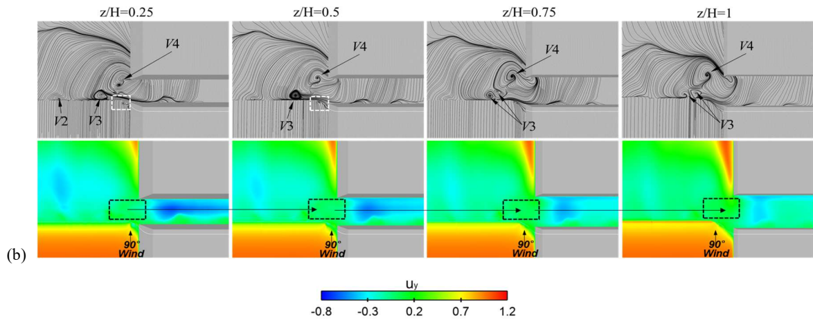
Figure 15. Streamlines and speed contours at different heights for wind angle of 90^\circ : (a) oblique structure (OS) transition and (b) circular curve structure (CCS) transition.
