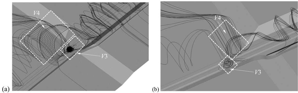
Figure 16. Streamlines for wind angle of 90^\circ : (a) OS transition and (b) CCS transition.
