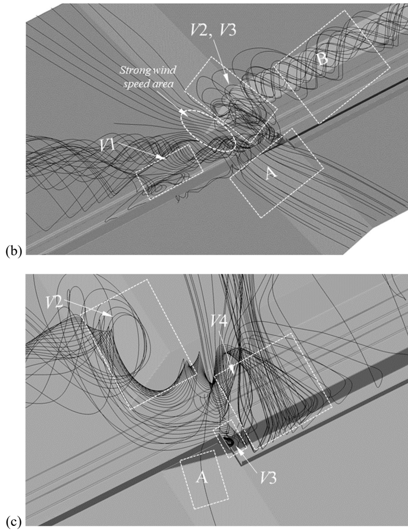
Figure 11. The space streamlines in the region of windbreak transition for wind angles of (a) 90^\circ , (b) 75^\circ and (c) 105^\circ .
