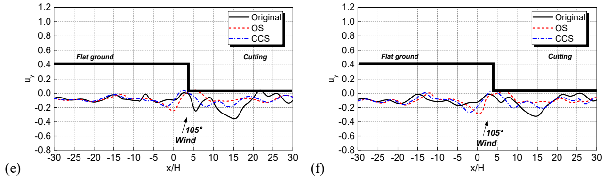
Figure 14. The wind speed along the railway: (a) RL-1 at 90°, (b) RL-2 at 90°, (c) RL-1 at 75°, (d) RL-2 at 75°, (e) RL-1 at 105° and (f) RL-2 at 105°.
