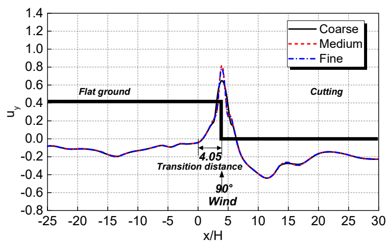
Figure 5. Result comparison between different meshes (“4.05” represents the transition distance x/H = 4.05 ).
