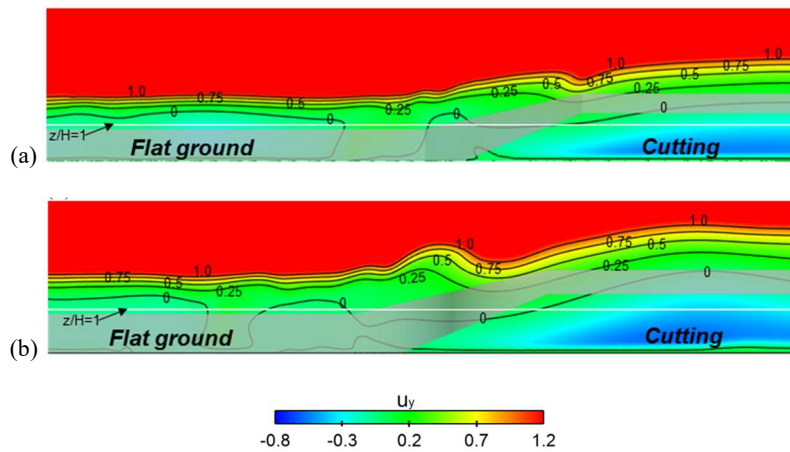
Figure 16. Streamlines for wind angle of 90^\circ : (a) OS transition and (b) CCS transition.
