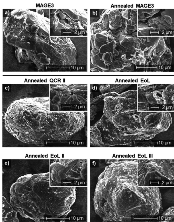
Fig. 9 Large 5000 \times magnified SEM images with 12000 \times magnified SEM images in the top right of each. (a) MAGE3 particle. (b) A particle of MAGE3 after annealing to 500 ^{\circ} C for 1 h. (c) QCR II (d) EoL (e) EoL II (f) EoL III. All AF were delaminated after 1 h of air exposure and annealing to 500 ^{\circ} C for 1 h.
