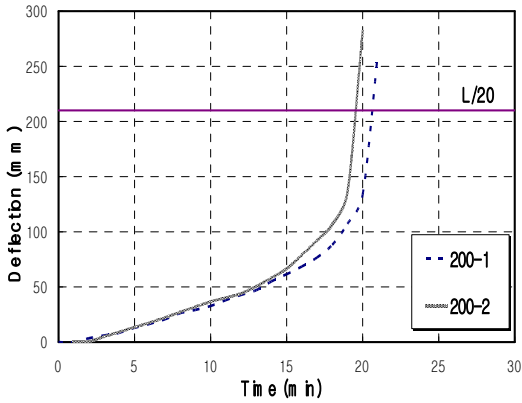
Figure 7. Relation of time and deflection (200 Series specimens)
