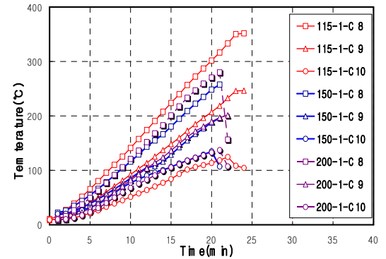
Figure 13. Relation of time and temperature (thermocouple no. 8~10 of composite ratio 30%)
