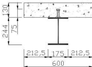
Figure 1. Detail of specimen
