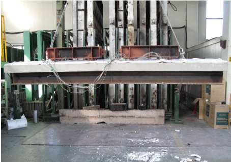
Figure 8. Photo of specimen before test
