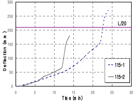
Figure 5. Relation of time and deflection (115 Series specimens)
