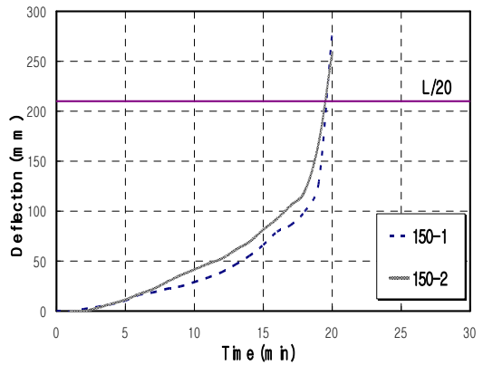
Figure 6. Relation of time and deflection (150 Series specimens)
