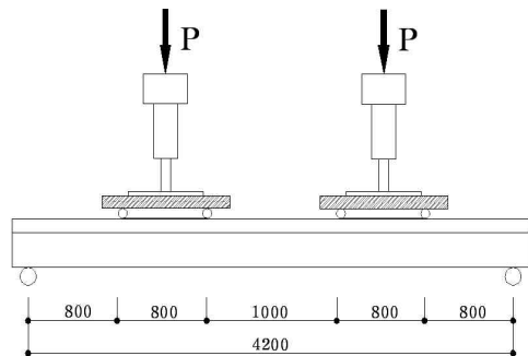
Figure 2. Test set up
