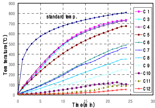
Figure 11. Temperature distribution of thermocouple at center location of beam
