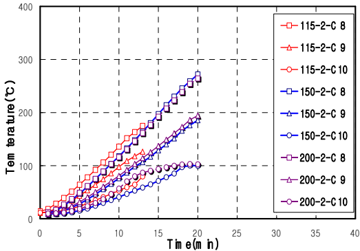
Figure 14. Relation of time and temperature (thermocouple no. 8~10 of composite ratio 60%)
