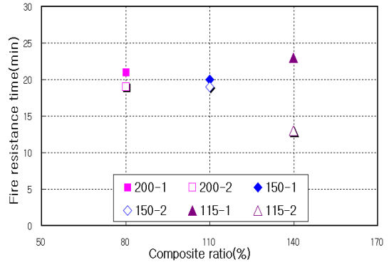
Figure 12. Relation of composite ratio and fire resistance time
