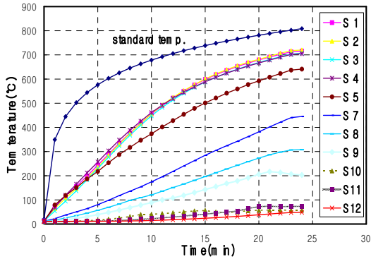
Figure 10. Temperature distribution of thermocouple at quarter location of beam
