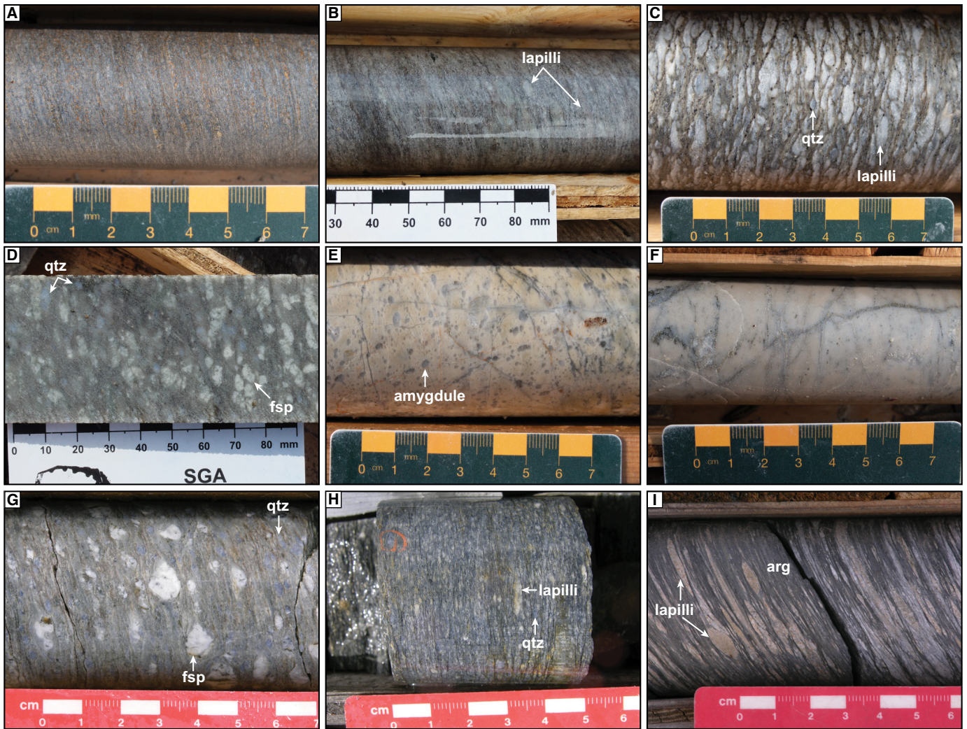
Fig. 9. Representative volcanic lithofacies in the Kudz Ze Kayah formation (A-F) and the Wolverine Lake group footwall (G-I). A) felsic tuff; B) matrix-supported felsic lapilli tuff; C) clast-supported felsic lapilli-crystal tuff, with blue quartz eyes; D) felsic crystal tuff with feldspar fragments and blue quartz eyes; E) amygdaloidal rhyolite; F) aphyric rhyolite; G) quartz-feldspar porphyritic intrusive rock, containing blue quartz and feldspar phenocrysts; H) felsic lapilli-crystal tuff with blue quartz eyes; I) tuffaceous argillite with lapilli. Abbreviations: Arg = argillite, fsp = feldspar, qtz = quartz.
