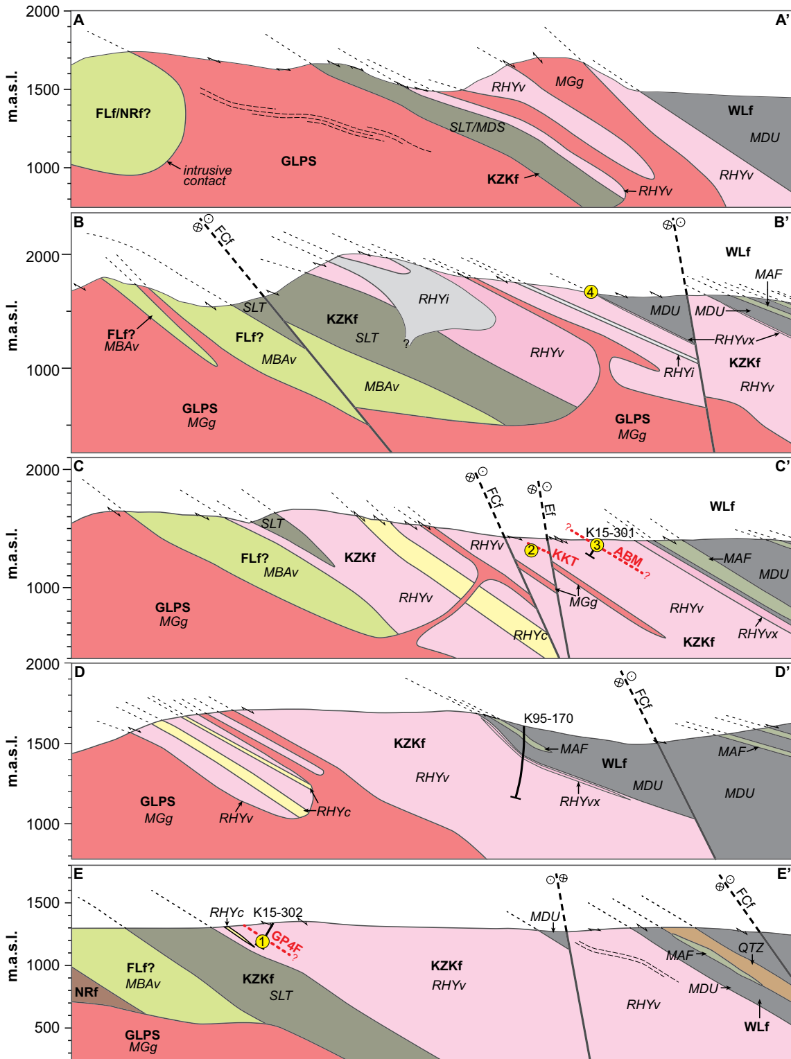
Fig. 6. Cross sections for lines A-A', B-B', C-C', D-D', and E-E' in the Kudz Ze Kayah formation, drafted with no vertical exaggeration. Sections correspond to plan view lines in Fig. 4. Unit colors and abbreviations as in the legend in Fig. 3. U-Pb samples are shown as yellow circles for reference and projected into the cross section where applicable (B-B' and C-C'; 17MM-002); numbers correspond to sample symbols in Figures 4 and 5. Thin, black dashed lines in the subsurface are interpreted cleavage plane variations based on outcrop measurements. Red dashed lines indicate approximate location of VMS lenses. Arrows on the surface indicate locations of outcrop measurements corrected as apparent dips. Abbreviations: Ef = East fault, FcF = Fault Creek fault, FLf = Fire Lake formation, GLPS = Grass Lakes plutonic suite, KKT = Krakatoa, KZKf = Kudz Ze Kayah formation, NRf = North River formation, WLf = Wind Lake formation.
