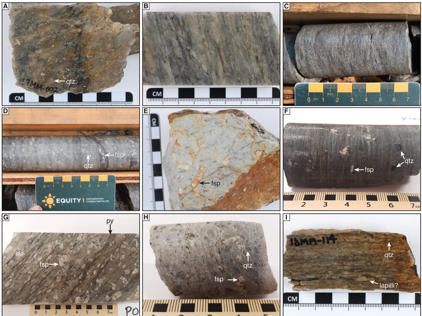
Fig. 11. Rock samples used for chemical abrasion-isotope dilution-thermal ionization mass spectrometry (CA-ID-TIMS) U-Pb zircon geochronology in the Kudz Ze Kayah formation (A-D) and the Wolverine Lake group (E-I). A) Felsic crystal tuff with blue quartz eyes located ~5 m below the Wind Lake-Kudz Ze Kayah formation contact (17MM-002). B) Felsic tuff to lapilli tuff in the hanging wall of the ABM zone (17MM-031). C) Felsic tuff with minor lapilli in the footwall of the Krakatoa horizon (18MM-133). D) Felsic crystal tuff with feldspar and blue quartz in the footwall of the GP4F deposit (17MM-074). E) Feldspar porphyritic intrusive rock in the Fisher zone (18MM-102). F) Felsic crystal tuff with feldspar and quartz fragments from the footwall of the Wolverine/Lynx zone (P99-WV-4K). G) Feldspar porphyritic intrusive rock from the footwall of the Wolverine/Lynx zone (P00-WV-1C). H) Quartz-feldspar porphyritic intrusive rock from the Sable zone (P00-WV-12). I) Felsic crystal tuff with quartz and feldspar in the lower Wolverine Lake group footwall (18MM-114). Mineral abbreviations: fsp = feldspar, py = pyrite, qtz = quartz.
