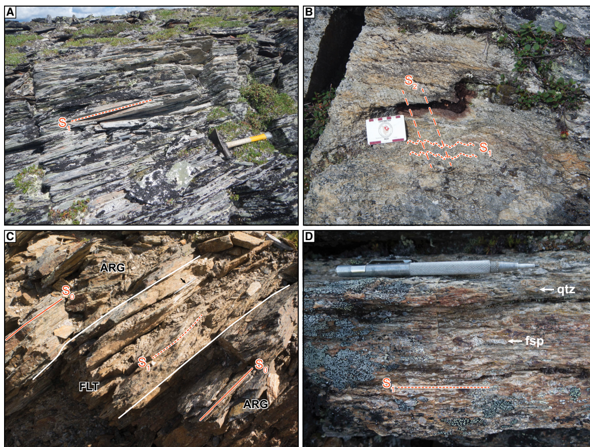
Fig. 10. Representative structural fabrics in the Kudz Ze Kayah formation (A-B) and the Wolverine Lake group footwall (C-D). Pervasive S_1 cleavage is the dominant planar feature in both geologic units. A) Prominent S_1 cleavage in an outcrop of felsic tuff, with a broadly west-east strike that dips to the north. B) Crenulation fabrics in a felsic tuff developed on an earlier S_1 cleavage, with a S_2 cleavage superimposed highly oblique to S_1 . C) Intercalated argillite (ARG) and felsic tuff (FLT) in the upper Wolverine Lake group footwall. Laminations of argillite beds represent primary bedding ( S_0 ), and S_1 cleavage in the FLT unit is subparallel to bedding. D) Quartz-feldspar porphyritic intrusive rock with strong mineral alignment subparallel to the prominent S_1 cleavage.
