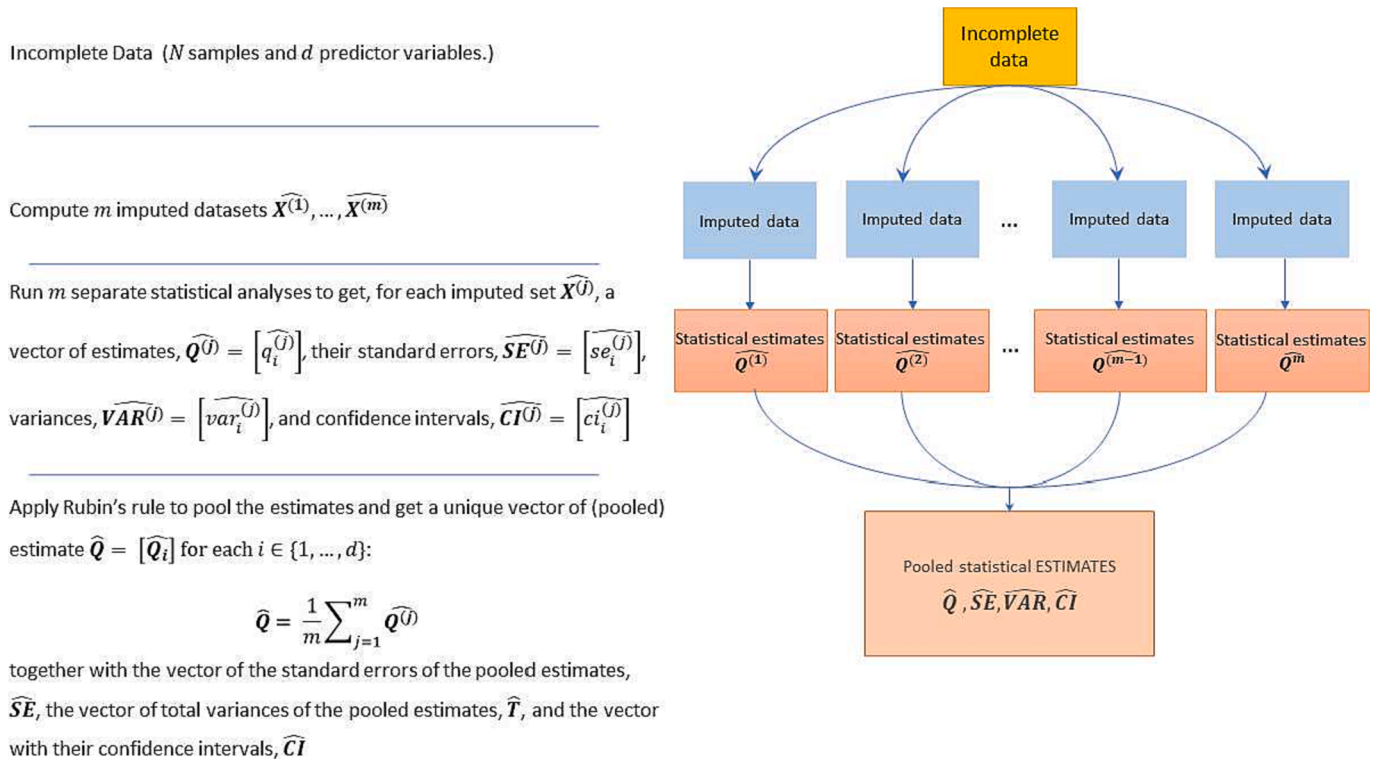
Fig. 2. Schematic diagram of the pipeline used to obtain pooled estimates when applying a MI strategy. The incomplete dataset is imputed m times, where the value of m can be defined in order to maximize the efficiency of the MI estimator (see App***endix A); each imputed dataset is individually processed to compute separate inferences; all the inferences are pooled by Rubin's rule [4] to get the pooled estimates ( \widehat{Q} ), their total variances ( \widehat{VAR} ) and standard errors ( \widehat{SE} ) and their confidence intervals ( \widehat{CI} ). In the figure, we use the superscript j to index the imputations number ( j \in \{1, \dots, m\} ) and the subscript i to index the predictor variable in the dataset (see Table 2 for a detailed list of all the notations used throughout the paper).
