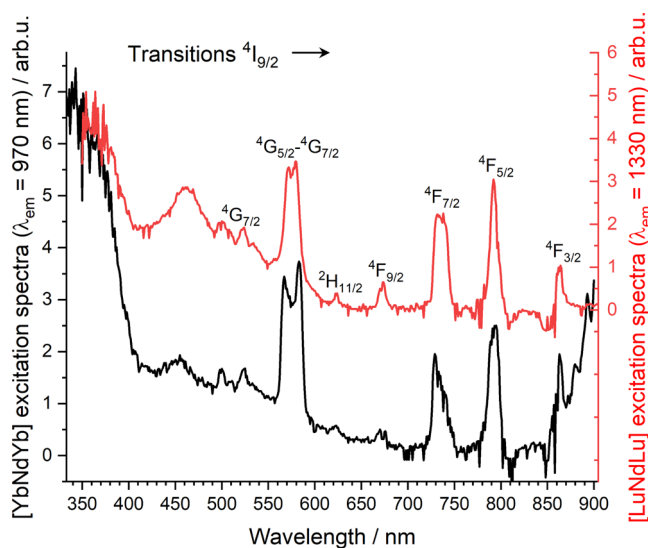
Figure 8. Excitation spectra of complex [LuNdLu] 3 (red trace) ( \lambda_{\text{em}} = 1330 \text{ nm} ) and complex [YbNdYb] 1 ( \lambda_{\text{em}} = 970 \text{ nm} ) in the solid state at 77 K.
