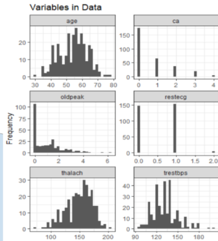
Fig. 2. Plot Variable 1
