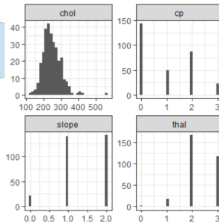
Fig. 3. Plot Variable 2
