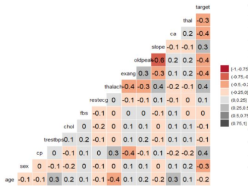
Fig. 4. Correlation Plot
