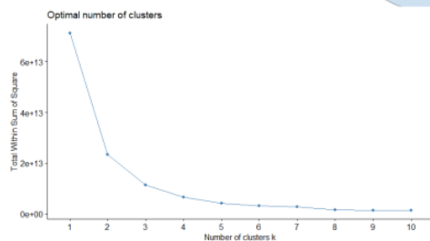
Gambar 4. Hasil clustering
