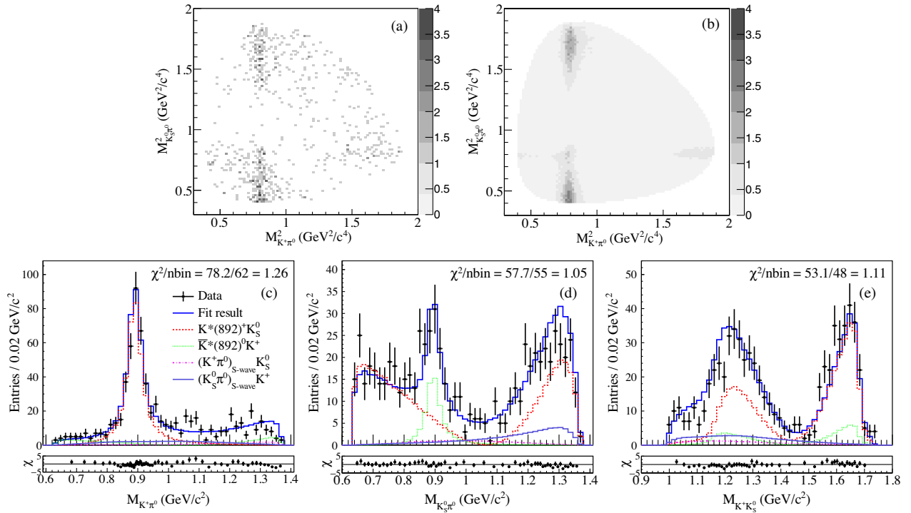
FIG. 4. The Dalitz plot distributions of (a) data and (b) nominal fit, along with the projections and corresponding pull distributions on (c) M_{K^+\pi^0} , (d) M_{K_S^0\pi^0} , and (e) M_{K^+K_S^0} of the nominal fit, where the black points with error bars denote data, the blue solid lines denote the fit results, and the other colored curves denote the different resonances components.
