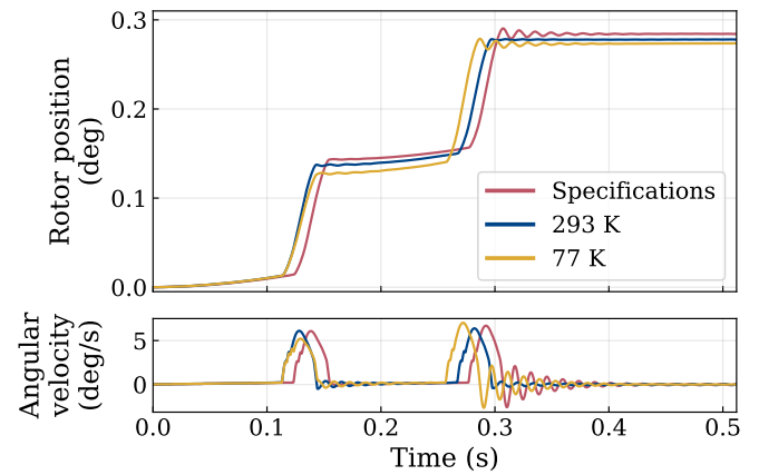
Figure 14: At low stepping frequencies (here: 100 Hz) the static friction included in the model produces a staircase like response. The input signal is the same as in Fig. 12 and \tau_{brk} = 90 mNm, \omega_{brk} = 10 deg/s and \tau_c = 0 . The number of steps changes with the value of \omega_{brk} .
