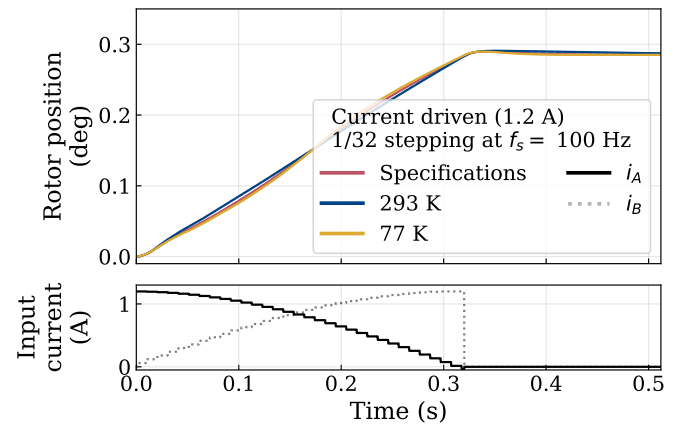
Figure 12: Similar to the left figure, but here at a much lower step frequency of 100 Hz, resulting in lower velocities and less overshoot.
