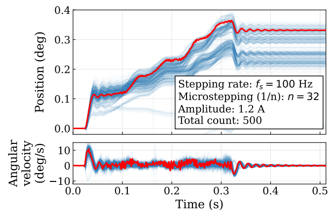
Figure 16: In this figure, the position and velocity of the ADC mechanism prototype is shown when a 100 Hz step frequency and 1/32 microstepping is used. The same staircase response occurs as in Fig. 14.
