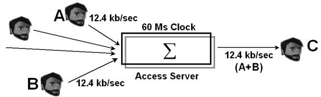
Figure 2. Multi-point, full duplex voice codec with additive bridging where the server can add incoming compressed streams from speakers A and B; f(A) + f(B) = f(A+B) .
