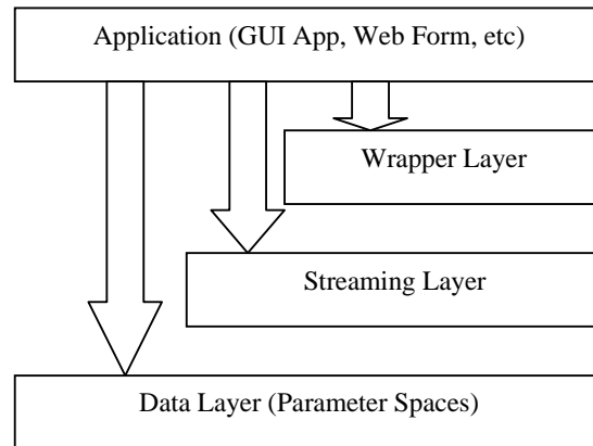
Figure 9. iFACE Layered Architecture
