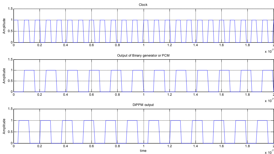
Fig. 5.1: Simulation's plots of clock (top trace), deterministic PCM (middle trace), deterministic DiPPM (bottom trace).
