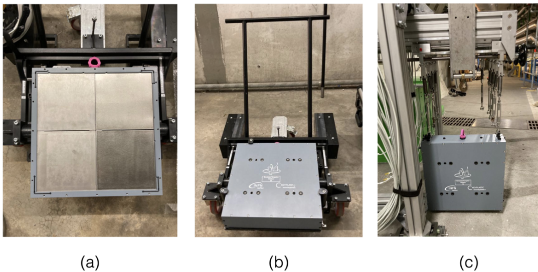
Figure 8: Target wall during the assembly with tungsten plates and emulsion films (a), on the transportation trolley (b) and suspended from the mechanical structure (c).
