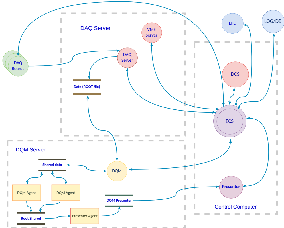
Figure 21: Simplified scheme of the SND@LHC online system.
