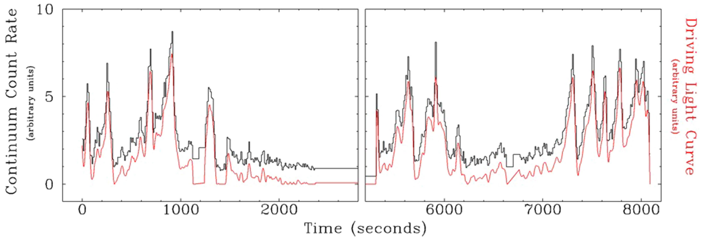
Extended Data Fig. 2 | The far-UV continuum and driving light curves. The black histogram shows the light curve of Swift J1858.6–0814 constructed from three broad wavelength regions that exclude the three strongest emission lines (N v \lambda 1240, Si IV \lambda 1400 and He II \lambda 1640). The specific regions used were \lambda 1290 Å–1390 Å, 1410 Å–1630 Å, 1660 Å–1850 Å. The light curve is shown normalized to an estimate of the underlying constant level ( 80 \text{ cs}^{-1} ).
