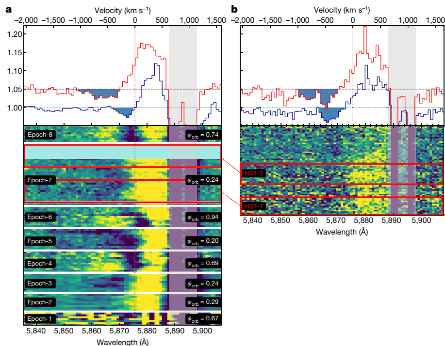
Fig. 2 | Apparently transient optical wind signatures. a , Trailed spectra of the eight GTC/OSIRIS epochs published in ref. 3 with the corresponding orbital phase 14 . b , VLT/X-Shooter during the HST visit centred on He I 5,876 Å. The average spectrum of all the observations is shown in the top panel with a blue line. Strictly simultaneous observations during the two UV exposures
