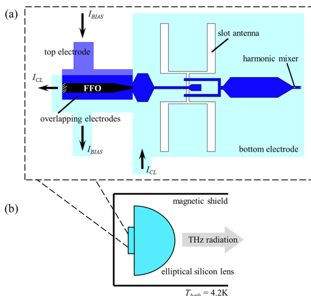
FIG. 1. (a) Layout of the planar microcircuit containing FFO, double-slot antenna, harmonic mixer, and the coupling structures between the elements. Both tunnel junctions, FFO and HM, are to be fabricated using Nb/AlN/NbN or Nb/ \text{AlO}_x /Nb trilayers in one technological process; top and bottom electrodes constitute the microstrip lines with an \text{SiO}_2 insulator layer. The full dimensions of the slot structure shown are 242 \times 90 \mu\text{m}^2 . (b) Scheme of the chip with the microcircuit shown in (a) placed at the far focus of the lens and inside the magnetic shield.
