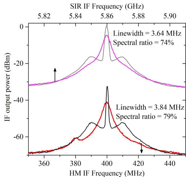
FIG. 6. Power spectra of the FFO at a frequency of 590 GHz for the sample with design #2 measured using the on-chip HM (SA #1)—free-running (red line) and phase-locked (black line) spectra, and measured using the SIR (SA #2)—free-running (magenta line) and phase-locked (gray line) spectra. The bottom and top axes of frequency represent the different IF ranges of 0–800 MHz for the on-chip HM IF and 4–8 GHz for the SIR IF. The span for both axes is the same, 100 MHz, and all the spectra are measured in the upper sideband. An estimated linewidth for the free-running spectra and a spectral ratio for the phase-locked spectra are shown near the curves. The resolution bandwidths of the analyzers are different: 1 MHz for SA #1 and 1.8 MHz for SA #2. For the spectra measured by SIR (magenta and gray lines), the LO of the SIR, FFO #2, is phase locked.
