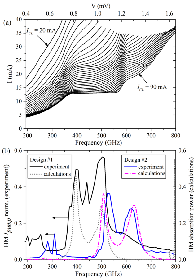
FIG. 5. (a) IVCs of the FFO with the dimensions 400 \times 16 \mu\text{m}^2 measured for different magnetic fields produced by the control line current with an I_{CL} step of 2 mA. (b) Experimental results of HM pumping by the FFO power and calculation results of the FFO power absorbed by the HM port. The HM I_{pump} is normalized to the “current jump” at the SIS gap voltage, equal to 206 \mu\text{A} for the HM in design #1 and 199 \mu\text{A} for the HM in design #2. The HM absorption power is normalized to the total FFO output power.
