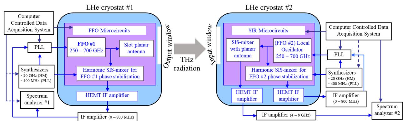
FIG. 4. Block diagram of the experimental setup for studying the FFO emission to open space using a THz spectrometer based on a superconducting integrated receiver.
