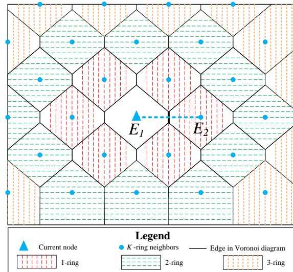
Figure 2. Voronoi diagram.
