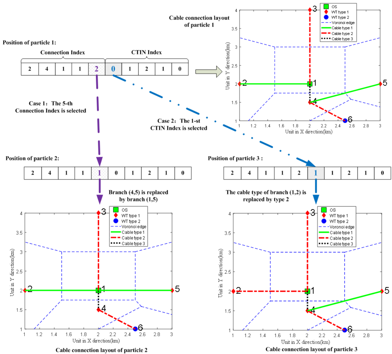
Figure 7. LSS for OWFD.
