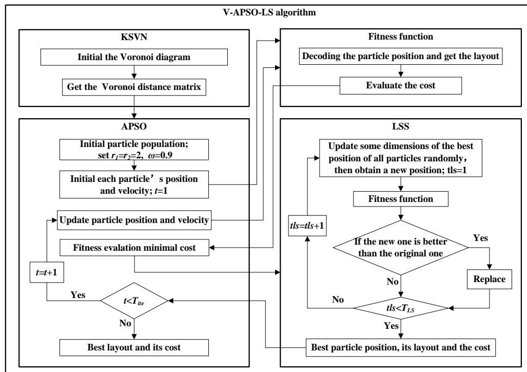
Figure 8. Optimization framework of V-APSO-LS.
