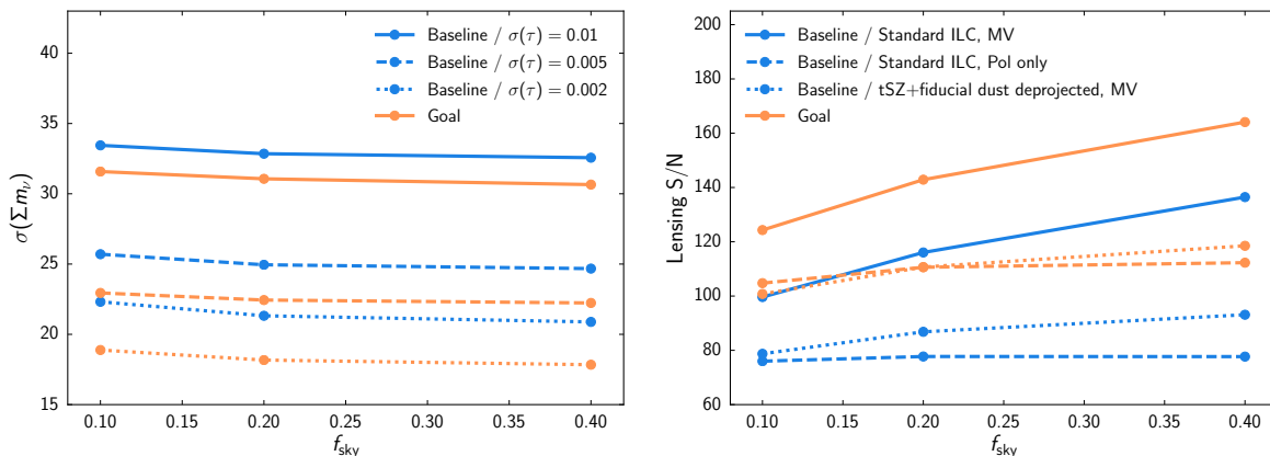
Figure 28. Left: neutrino mass constraints from temperature and polarization CMB power spectra and lensing potential autospectrum, including foreground cleaning with explicit tSZ deprojection for temperature and dust deprojection for polarization, as a function of sky area. Right: lensing potential autospectrum signal-to-noise ratio from temperature and polarization CMB data as a function of sky area. Foreground cleaning is included with standard ILC without explicit deprojection (Deproj-0) or tSZ deprojection for temperature and dust deprojection for polarization (Deproj-1), as discussed in section 2.5.1.
