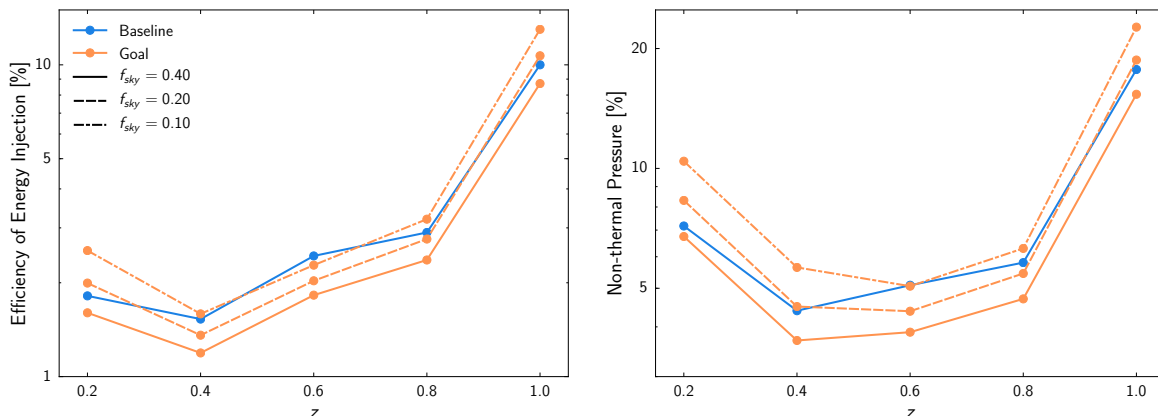
Figure 37. Forecast 1\sigma uncertainties on the feedback efficiency, \epsilon , (left) and the non-thermal pressure support, \alpha , (right) using SO combined with DESI Luminous Red Galaxies, through cross correlating the thermal and kinematic Sunyaev-Zel’dovich effects. Different colors distinguish between baseline and goal sensitivities and different line styles show the impact of different sky coverages.
