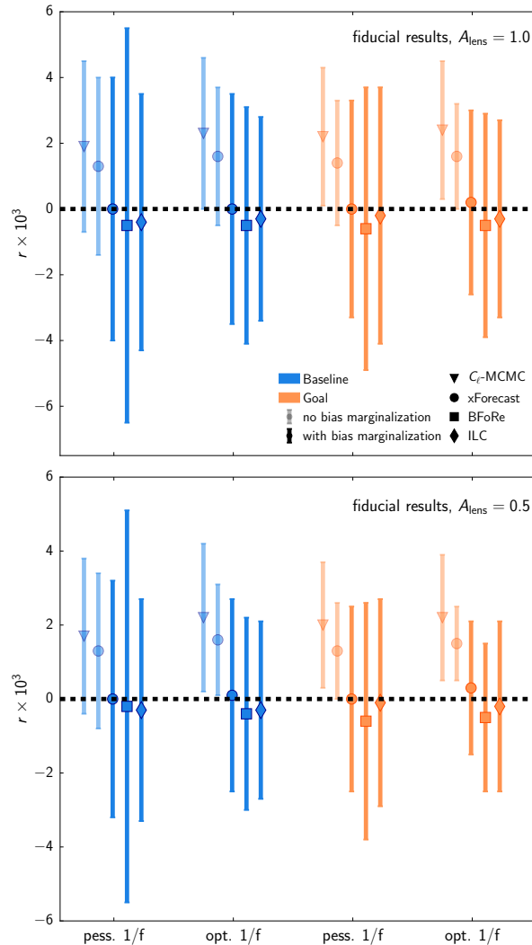
Figure 10. Estimated r and 1\sigma uncertainties for simulations with r = 0 and A_{\text{lens}} = 1 (top) and 0.5 (bottom). The fiducial sky model has single dust and synchrotron components with spatially varying spectral indices, described in section 2.4.4. We show baseline and goal noise levels, with either pessimistic or optimistic 1/f scenarios, for the C_\ell -MCMC and \text{xForecast} methods, without residual marginalization (translucent), and for the \text{xForecast} , BFoRe and ILC methods that additionally marginalize over foreground residuals at the power spectrum level (solid).
