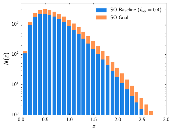
Figure 33. The forecast SZ cluster abundances as a function of redshift for the SO baseline and goal configurations with f_{\text{sky}} = 0.4 in bins of redshift with width \Delta z = 0.1 and a S/N > 5 . We forecast approximately 16,000 clusters with baseline noise levels and approximately 24,000 clusters with the goal noise levels.
