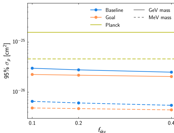
Figure 25. We show current 95% confidence-level upper limits on the cross section for dark matter-proton elastic scattering, derived using Planck temperature, polarization, and lensing anisotropy measurements ([122], yellow lines) assuming a velocity-independent spin-independent interaction. Limits for dark matter masses of 1 GeV and 1 MeV are shown as horizontal solid and dashed line, respectively. We also show the projected limits for the baseline and goal SO LAT configurations, as a function of the fractional sky coverage, for the same two masses. We see an improvement of a factor of 7.6 in constraining power for SO with f_{\text{sky}} = 0.4 , over Planck .
