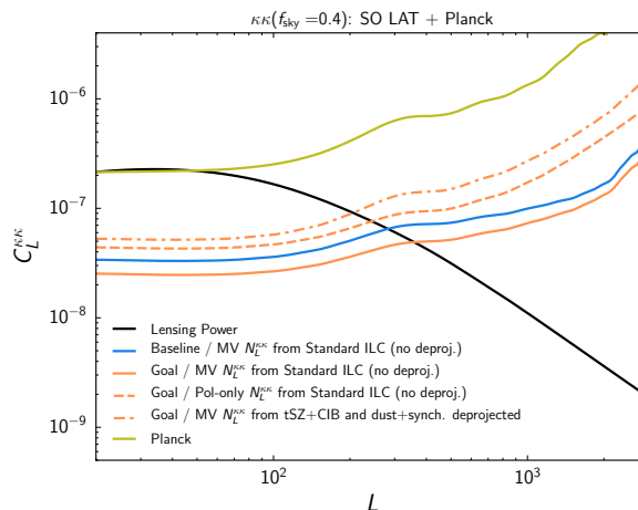
Figure 6. \Lambda CDM CMB lensing power spectrum (black) compared to SO LAT lensing noise curves, N_L^{\kappa\kappa} , reconstructed assuming a polarization only (Pol-only) or minimum variance (MV) combination of estimators in the case of standard ILC for both CMB temperature and polarization cleaning (solid and dashed curves), and tSZ and fiducial CIB SED deprojection for CMB temperature cleaning and fiducial polarized dust and synchrotron SED deprojection for CMB polarization cleaning (dot-dashed curve). SO baseline and goal scenarios are shown in blue and orange, respectively, and compared to the Planck lensing noise ([288], yellow). SO will be able to map lensing modes with S/N > 1 to L > 200 .
