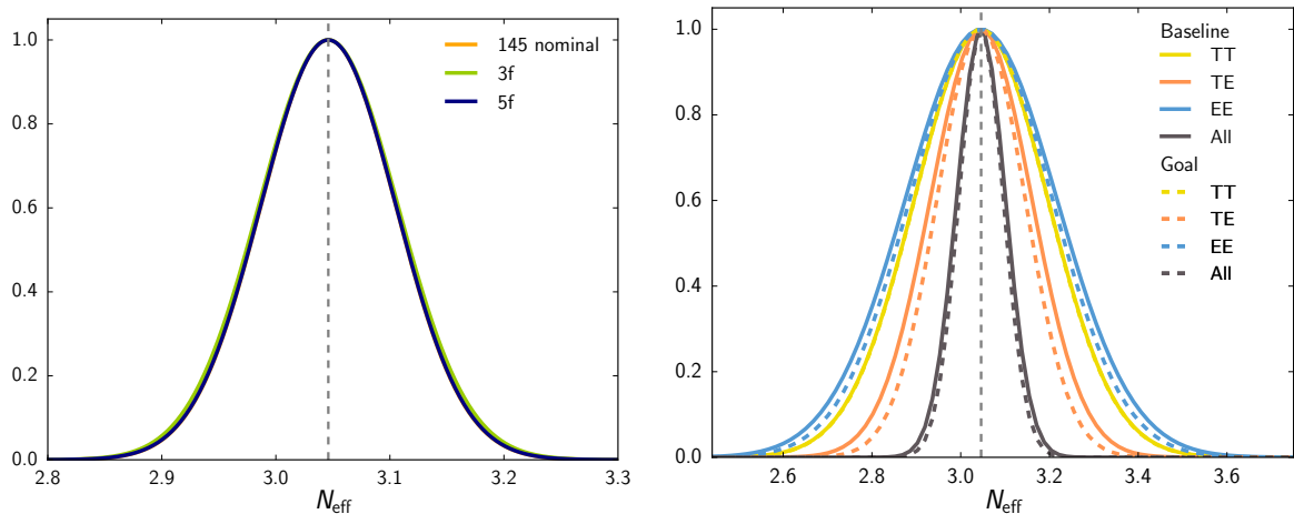
Figure 18. Left: impact of foreground cleaning the LAT using 5 (blue) or 3 (green) frequencies on the N_{\text{eff}} estimate. The 145 nominal orange curve shows the result assuming the ideal case of having no foregrounds in the data. The gain from retaining frequency information is completely negligible. Right: constraints on N_{\text{eff}} from individual small-scale spectra ( TT , TE , EE ) and the total, shown for baseline (solid) and goal (dashed) scenarios. The most constraining channel is the foreground-clean TE spectrum.
