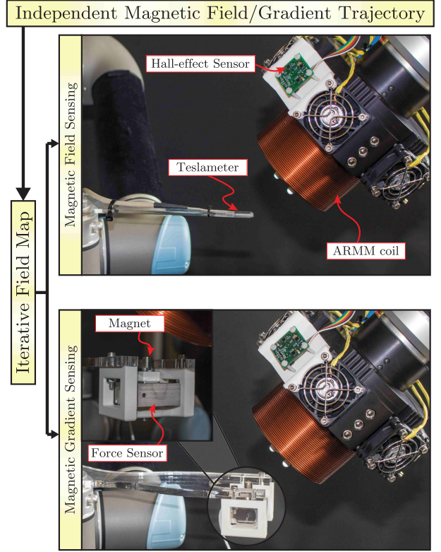
Fig. 7. Setup used to validate the iterative map proposed in Section III. In this experiment, the ARMM system is used to generate prescribed magnetic field/gradient trajectories for a selected point ( \mathbf{p} \in \mathbb{R}^3 ). Initially, a Senis 3MH3A-500MT (Senis AG, Baar, Switzerland) teslameter is used to sense the magnetic field at \mathbf{p} for the duration of the trajectory. Following that, the teslameter is replaced by a permanent dipole with known magnetic dipole moment ( \mu ) attached to a K3D40 force sensor (Meßsysteme AG, Henningsdorf, Germany) and the trajectory is repeated. The measurements from the force sensor are processed to recreate the magnetic field gradient generated by ARMM. Both sensors are precisely positioned at \mathbf{p} using the UR5 robotic arm (Universal Robots, Odense, Denmark) to ensure that the measurements are taken in the same location.
