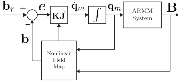
Fig. 6. ARMM system employs an iterative field map to generate reference magnetic field and its gradient \mathbf{b}_r = [B_r (\partial B_r / \partial z)]^T at \mathbf{p} . The information about the configuration ( \mathbf{q}_m = [z I]^T ) of the system, as well as measurements from magnetic field sensor are used to generate an error signal ( \mathbf{e} \in \mathbb{R}^2 ). The error is minimized using a Jacobian inverse scheme, employing the derivation presented in (15). \dagger denotes damped pseudo-inverse, used in place of regular matrix inverse for improved stability [27]. The gain ( \mathbf{K} \in \mathbb{R}^{2 \times 2} : \mathbf{K} > 0 ) of the scheme is tuned manually until satisfactory performance is achieved.
