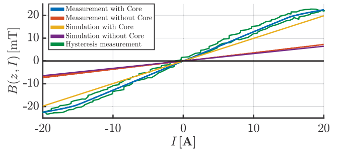
Fig. 5. Senis 3MH3A-500MT (Senis AG, Baar, Switzerland) teslameter is used to measure the value of the magnetic field ( B(z, I) ) generated by the coil of the ARMM system at the location ( z = 10 cm) in the entire operational range of current ( I ). The results are compared to predictions from the FE model used in the design process. The measurements and simulations are performed for the coil with and without the Vacoflux core. The graph shows that the coil produces more magnetic field than predicted by the model. This is mostly due to the better magnetic properties of the core. Furthermore, an additional fast sweep (green) across the entire operational current range in 0.5 s. This was performed to investigate the presence of hysteretic behavior during sudden current variations, as motivated by our previous experience with similar electromagnets. Limited hysteretic behavior is observed. However, since such sudden variations in current are unlikely to occur during catheter steering tasks, we neglect this behavior. Nevertheless, the coil exhibits saturation in the operational range. As this phenomenon makes the actuation non-linear for any rate of current, it needs to be taken into account while using ARMM for precise magnetic actuation.
