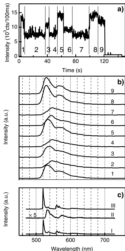
FIG. 4. Temporal variations of the electronic coupling strength of individual BPM dimers. (a) Fluorescence intensity trajectory of a single BPM dimer. (b) Fluorescence spectra recorded during the time intervals numbered correspondingly in (a). The fluctuations in spectral shape and position reflect transitions between localized (1, 3, 5, 8, 9) and delocalized states (2, 4, 6, 7) of the dimer. These measurements have been conducted at room temperature. (c) Fluorescence spectra of a single BPM dimer recorded at 1.4 K. Again spectral fluctuations are observed as a function of time (I: t = 0 s; II: t = 40 s; III: t = 80 s).
