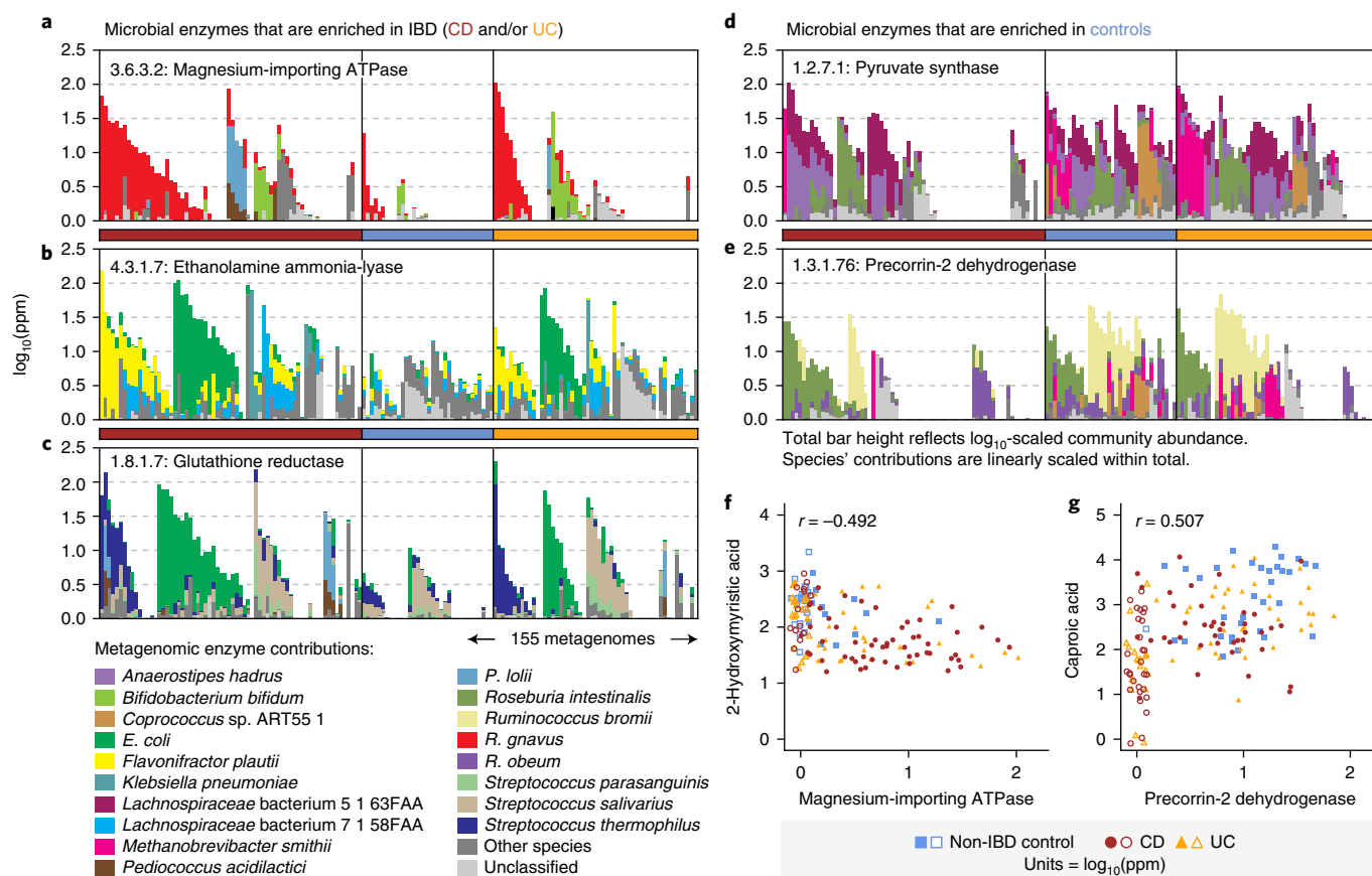
Fig. 5 | IBD-associated changes in microbial function and their metabolic associations. a–e , Examples of metagenomically contributed enzymes that were differentially abundant in IBD, annotated by their taxonomic contributors ( a–c are enriched in IBD; d and e are depleted). In each case, the enzyme was contributed by a mixture of species across the cohort, and not dominated by a single species. Each set of stacked bars represents one of the 155 PRISM metagenomes (arrayed on horizontal axes). Community enzyme abundance ( \log_{10} -transformed ppm) is represented by the top of each stack of bars; contributions from major species are linearly scaled within the total bar height. Samples were first sorted according to the dominant contributor to a function and then grouped by phenotype (sample ordering differs between panels). f, g , Correlations between community total enzyme abundance and IBD-associated metabolites across 68 CD and 53 UC patients and 34 non-IBD controls. Values plotted are raw measurements (not residuals) normalized to ppm units and then \log_{10} -transformed. Values <1 ppm (including 0s) were set to 1 ppm for plotting; corresponding points are shown without fill and jittered (all other points have a solid fill). The given r values indicate Spearman's rank correlation.
