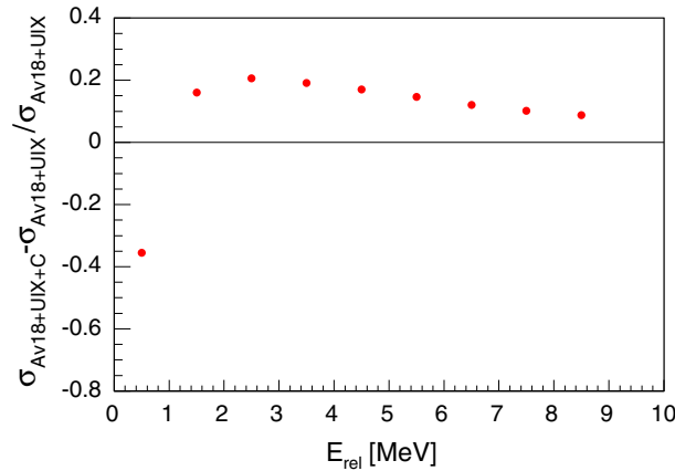
Fig. 3 Net effect of the Coulomb force on the theoretical breakup cross section at 65 MeV/nucleon presented as function of the E_{rel} variable. The calculations are matched to the acceptance of the GeWall detector
