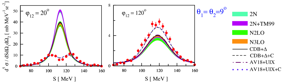
Fig. 1 Differential cross-section data for the d - p breakup reaction at 130 MeV at two different kinematical configurations (specified in the panels ) in which significant Coulomb force effects are observed. The data are compared to various theoretical calculations, described in the legend
