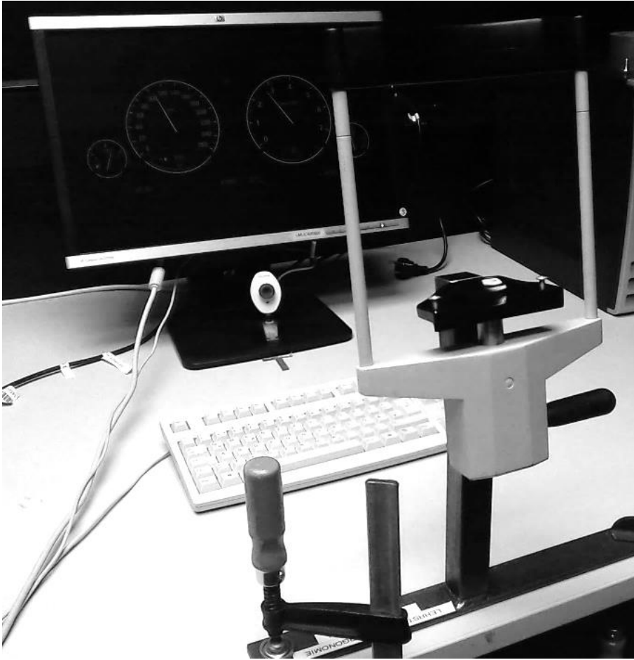
Figure 3 Setup of the occlusion task with a screen in front of the participants and a chin rest for the head.
