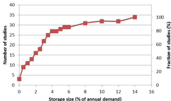
Fig. 5. Storage energy size as a function of VRE penetration for systems with less than 100% RES.
