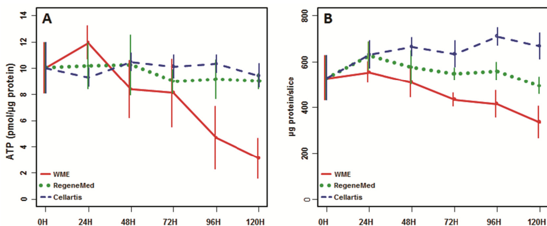
Figure 1. ATP (A) and protein (B) content in hPCLS during 120 h incubation in three different media (WME (red line), RegeneMed ® (green dotted line) and Cellartis ® (blue dashed line)). Data represent the average \pm SEM of 4 experiments (4 different livers), using 3 hPCLS for each group in every experiment.
