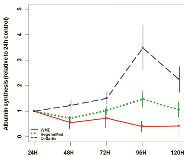
Figure 6. Albumin synthesis over time by hPCLS incubated in WME (red line), RegeneMed ® (green dotted line) or Cellartis ® (blue dashed line). Data are expressed as relative value to 24h control ( \pm SEM).
