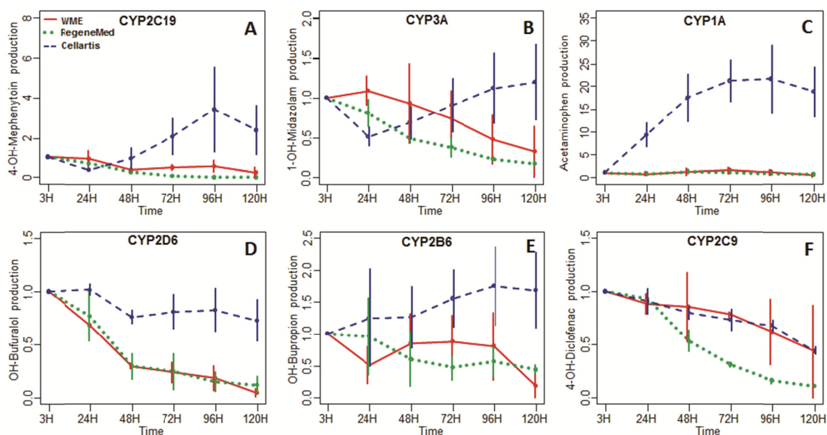
Figure 4. Phase I metabolite production of mephenytoin (A), midazolam (B), phenacetin (C), bufuralol (D), bupropion (E) and diclofenac (F) during 5 days by hPCLS incubated in WME (red line), RegeneMed ® (green dotted line) and Cellartis ® (blue dashed line). Data are expressed as relative values \pm SEM to the value at 0-3h incubation. 3 (WME and Cellartis ® ) or 2 (RegeneMed ® ) donor livers were used for each study, using 3 hPCLS for each group in every experiment.
