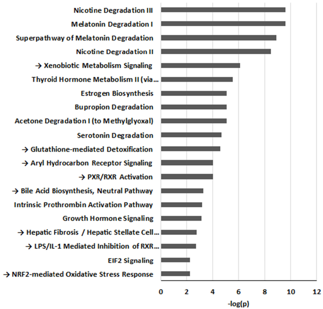
Figure 7. Top 20 significantly regulated pathways in hPCLS following 5 days of incubation.
