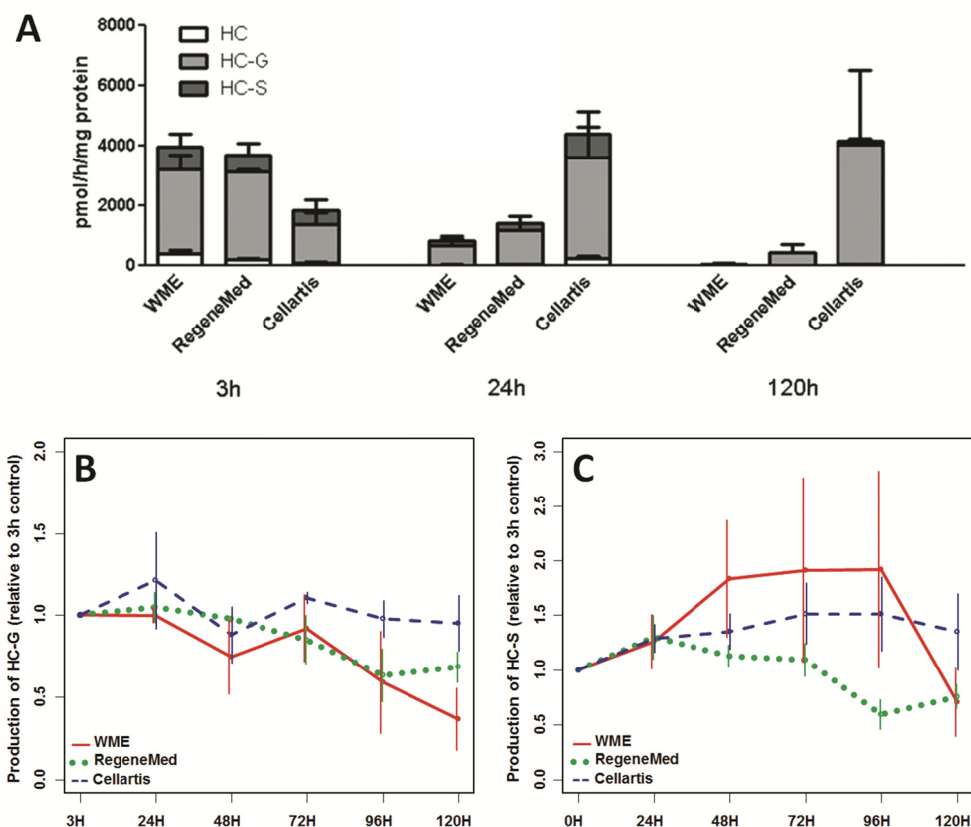
Figure 5. Phase I and II metabolism of 7-EC (A) and Phase II metabolism of 7-HC (B, C) during 5 days by hPCLS incubated in WME (red line), RegeneMed ® (green dotted line) and Cellartis ® (blue dashed line). Data are expressed as relative values ( \pm SEM) to the value at 0-3h incubation.
