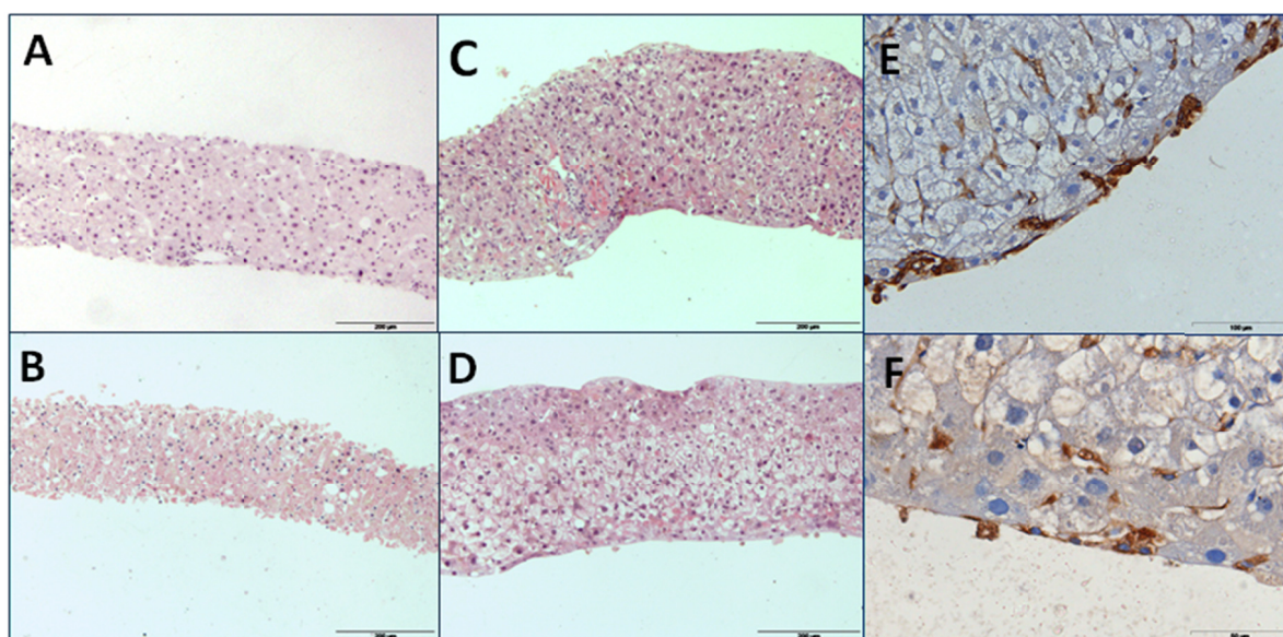
Figure 2. Hematoxylin-eosin staining of cross-sections of hPCLS at 0h (A) and incubated 120h in WME (B), RegeneMed ® (C) or Cellartis ® (D). Vimentin staining of the new cell layer around the slice incubated for 120h in RegeneMed ® (E) or Cellartis ® (F). Representative images are shown. Scale bar = 200 μm for A-D, 100 μm for E and 50 μm for F.
