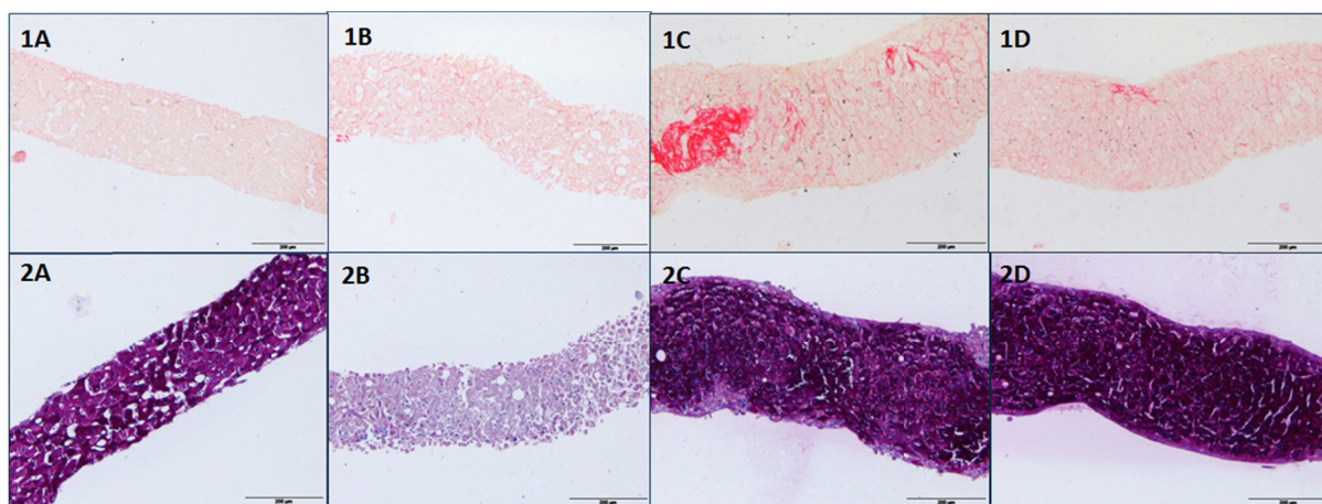
Figure 3. Cross-sections of hPCLS at 0h (A) and incubated 120h in WME (B), RegeneMed ® (C) or Cellartis ® (D) stained with Sirius Red (1) or PAS (2). Representative images are shown. Scale bar = 200 μm.
