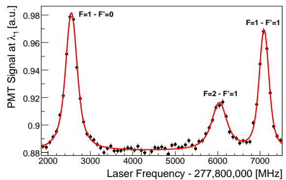
FIG. 3: HFS of the 6^2D_{3/2} - 7^2P_{1/2} transition in ^{213}\text{Ra}^+ . The solid line represents a fit of three Voigt profiles to the data. One parameter is used to fit the Gaussian widths of the three resonances, which yields a FWHM of 181(20) MHz. The Lorentzian widths (FWHM) are 245(20), 368(70), and 147(9) MHz (left to right). The different Lorentzian widths are due to saturation effects. The fit has a reduced \chi^2 = 1.1 at 62 degrees of freedom.
