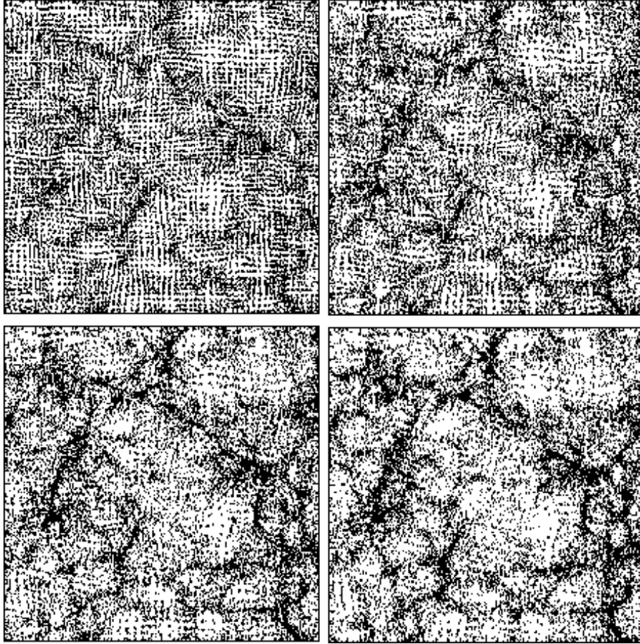
Figure 21. Zel’dovich displaced particle distributions inferred from a unconstrained random realization of a primordial matter distribution for a SCDM cosmological scenario in a 50h^{-1}\text{Mpc} box. Time sequence from top left to bottom right, frames corresponding to cosmic epochs a = 0.10, 0.15, 0.20 and 0.25 .
