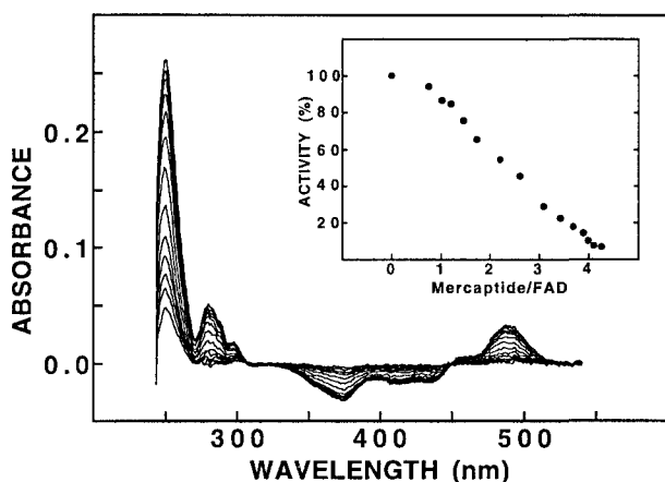
Fig. 2. Difference spectra observed during the inactivation of 10 \mu M VAO by 125 \mu M 4-hydroxymercuribenzoate in 50 mM Hepes, pH 7.5. Spectra are shown, recorded 1, 3, 5, 8, 12, 19, 31, 47, 61, 75, 90, 105 and 120 min after mixing. Inset: The formation of mercaptide bonds is plotted as a function of residual VAO activity.
