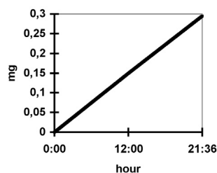
Figure 4: Performance of the pulse-free disposable syringe pump at 300 \text{nl}\cdot\text{min}^{-1} .
