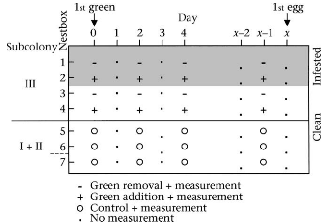
Figure 1. Schematic design to test the nest protection function of green nesting material. In subcolony III sets of four nestboxes (two infested and two clean) were selected, such that the first green material appeared in all four nestboxes on the same day (day = 0). Each nestbox was subjected to either a green removal or a green addition treatment every other day until one of the nestboxes contained an egg (day = x). As a control treatment, five sets comprising two or three clean nestboxes from subcolonies I and II were selected such that the green nest material was not manipulated and that the date of first appearance of green material in the control set was similar to that of one experimental set. The dashed line indicates that some sets comprised two and others three control nestboxes.
