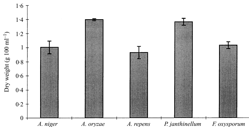
Fig. 6. Effect of silicic acid on growth of fungi in unbuffered Czapek Dox medium, expressed as increase in dry weight after subtraction of the weight of the control for each individual fungus. (All increases were significant at P < 0.05 ).
