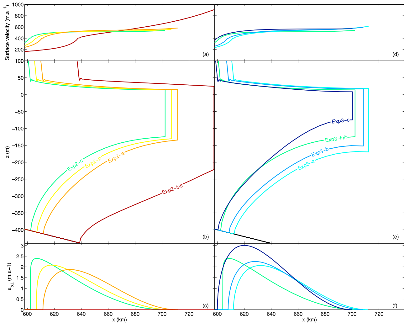
Figure 1. Surface velocity, geometry and corresponding sub ice-shelf melt distribution for the steady ice-shelf with lateral friction and different melt distribution. Exp2: (a–c), steady state solutions obtained without melting (red curve) and for different melting distributions \beta = 1.5 (orange), \beta = 1.25 (yellow), \beta = 1.1 (green) with the same average basal melt rate \bar{a}_{b\perp} = 1.0 \text{ m a}^{-1} ; Exp3 (d–e), starting from the solution for \bar{a}_{b\perp} = 1.0 \text{ m a}^{-1} and \beta = 1.1 (green curve), steady state solutions obtained after a change of the shape of the melting rate distribution ( \beta = 1.5 ) and an increase of the average melt rate to \bar{a}_{b\perp} = 1.1 \text{ m a}^{-1} (light blue), \bar{a}_{b\perp} = 1.2 \text{ m a}^{-1} (blue) and \bar{a}_{b\perp} = 1.6 \text{ m a}^{-1} (dark blue).
