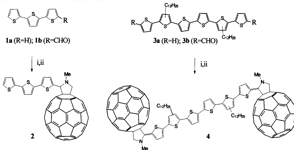
FIGURE 1. Synthesis of oligothiophene-fullerene dyads. Step i: DMF, \text{POCl}_3 ; step ii: N-methylglycine, C_{60} , toluene, \Delta .
