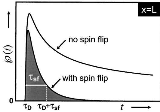
FIG. 3. Probability per unit volume that, once an electron is injected, will be present at x=L without spin flip [ \varphi(t) ] and with spin flip [ \varphi(t) \times \exp(-t/\tau_{sf}) ], as a function of the diffusion time t .
