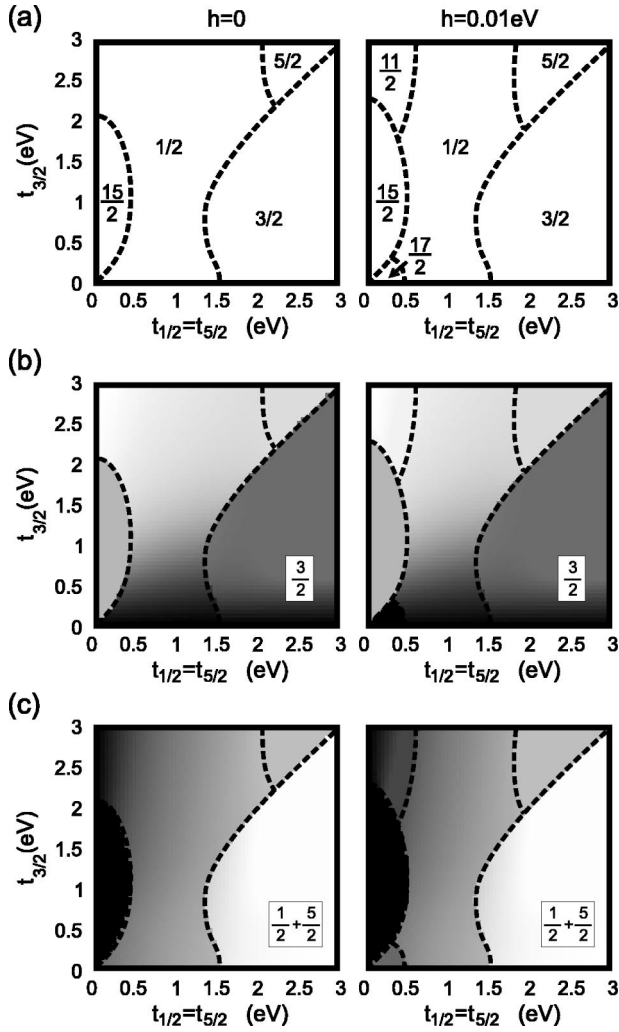
FIG. 8. Phase diagram for the Gutzwiller wave function in the t_{1/2} - t_{3/2} plane (with t_{1/2}=t_{5/2} ) for vanishing (left) and finite (right) ferromagnetic fields. (a) Phases are characterized by their \mathcal{J}_z expectation value. (b) Ratio T_{3/2}/t_{3/2} as gray-scale plots (black—0, white—1.4) and (c) the sum of the corresponding ratios for j_z = 1/2 and 5/2 (black—0, white—2.4). In comparison with Fig. 2, note the different plot ranges.
