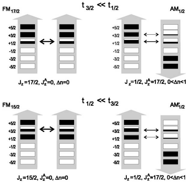
FIG. 4. Configurations relevant for weakly anisotropic hopping (hybridization) in the presence of ferromagnetic (FM, left column) and antiferromagnetic (AM, right column) fields for t_{3/2} \ll t_{1/2} = t_{5/2} (top row) and t_{1/2} = t_{5/2} \ll t_{3/2} (bottom row). Rectangles symbolize the j_z orbitals on both sites, with black areas presenting their occupation. The thickness of horizontal arrows between orbitals symbolizes their contributions to the kinetic-energy gain. The arrow-shaped background emphasizes the role of the fields. Note the charge disproportionation 0 < \Delta n_f < 1 in the antiferromagnetically aligned states.
