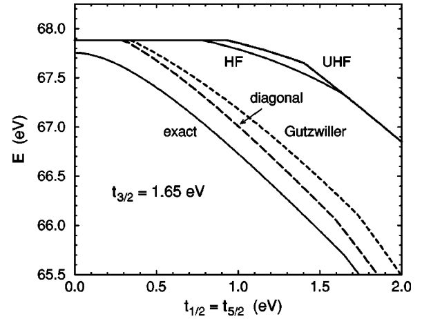
FIG. 9. Total energies for various approximation as a function of t_{1/2}=t_{5/2} at fixed t_{3/2}=1.65 eV: (exact) numerical diagonalization of the 600 \times 600 matrix, see Fig. 1; (diagonal) diagonalization keeping only the diagonal interaction matrix elements, see Fig. 2; (HF) Hartree-Fock approximation, see Fig. 3; (UHF) unrestricted Hartree-Fock approximation, see Fig. 7; (Gutzwiller) variational wave function (17), see Fig. 8.
