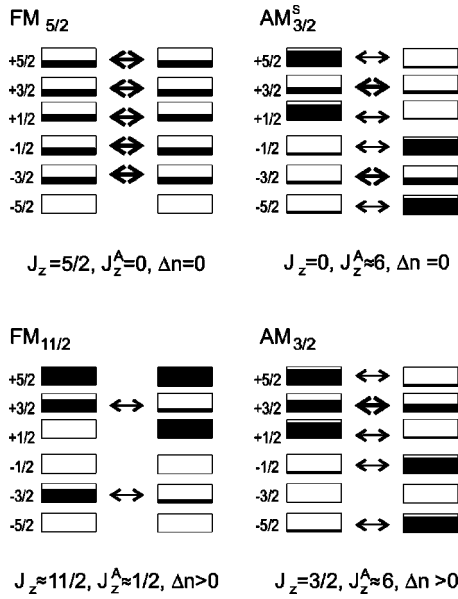
FIG. 5. Configurations relevant for large hopping: The upper left panel ( FM_{5/2} ) shows an overall ferromagnetic arrangement with all electrons contributing to the kinetic-energy gain. The upper right panel ( AM_{3/2}^S ) presents an overall antiferromagnetic arrangement dominated by t_{3/2} hopping which is symmetric with respect to the site index. t_{3/2} hopping dominates also in the lower row. In the lower left panel ( FM_{11/2} ), the overall arrangement is of ferromagnetic type, whereas in the lower right panel ( AM_{3/2} ) it is of antiferromagnetic character. As in Fig. 4, black areas symbolize the orbital occupation and the linewidth of the arrows symbolize the corresponding contributions to the kinetic-energy gain. Field directions are not indicated, in order to emphasize the dominant role of the hopping for the formation of these states.
