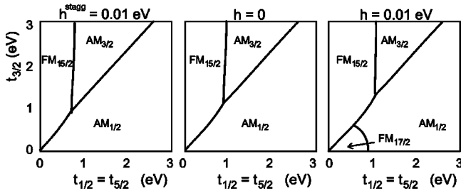
FIG. 7. Hartree-Fock approximation with variational space restricted to j_z eigenstates (UHF): Phase diagram in the t_{1/2} - t_{3/2} plane ( t_{1/2}=t_{5/2} ) with ferromagnetic (right), vanishing (middle), and antiferromagnetic (left) fields. The phases are characterized from the z components of the angular momentum and the state occupation, cf. Figs. 4 and 5.
