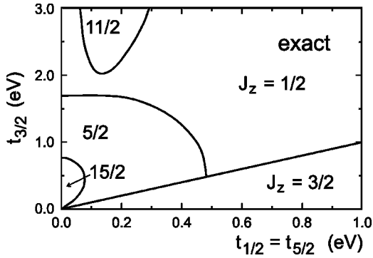
FIG. 1. Phase diagram for the f^2 - f^3 model of Ref. 14 in the t_{1/2} - t_{3/2} plane ( t_{5/2}=t_{1/2} ), derived from the total magnetization \mathcal{J}_z ( z component of the total angular momentum) of the ground state for infinitesimal field h_n=0^+ . Numbers indicate \mathcal{J}_z , which is a good quantum number.
