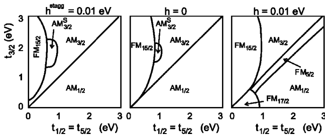
FIG. 3. Phase diagram in the t_{1/2} - t_{3/2} plane (with t_{1/2} = t_{5/2} ) in the Hartree-Fock approximation with ferromagnetic (right), vanishing (middle), and antiferromagnetic (left) fields. The phases are characterized from the z components of the angular momentum and the state occupation and labeled according to the notation of Figs. 4 and 5.
