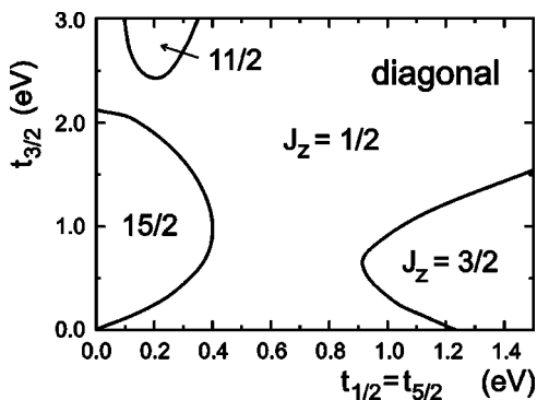
FIG. 2. Phase diagram within the diagonal approximation (7) in the t_{1/2} - t_{3/2} plane ( t_{1/2}=t_{5/2} ), derived from the total magnetization \mathcal{J}_z of the ground state for infinitesimal field h_n=0^+ . In comparison with Fig. 1, note the different plot ranges.
