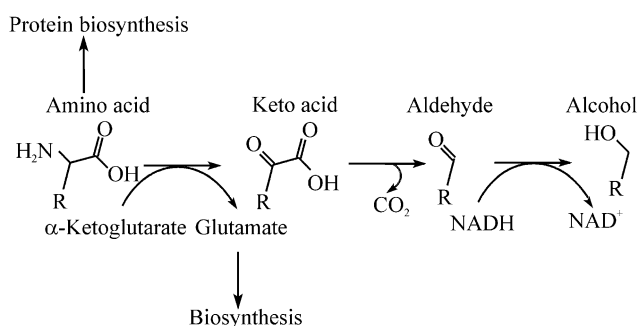
Fig. 1. The Ehrlich pathway [3,4]. A schematic representation of the conversion of branched-chain amino acids to fusel alcohols; leucine via \alpha -keto isocaproate and 3-methylbutyraldehyde to isoamyl alcohol; isoleucine via \alpha -keto- \beta -methylvalerate and 2-methylbutyraldehyde to active amyl alcohol; valine via \alpha -ketoisovalerate and isobutyraldehyde to isobutyl alcohol (valine: R = C 3 H 7 , leucine and isoleucine: R = C 4 H 7 ).
