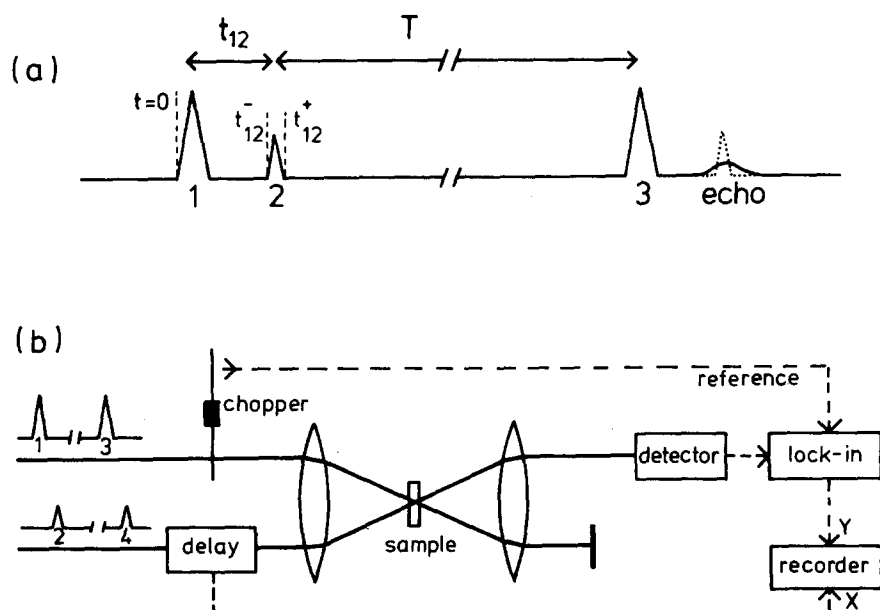
FIG. 1. Schematics of the experimental setup for the detection of photon echoes simulated from an accumulated grating. Note that the echo in time overlaps with a probe pulse.
