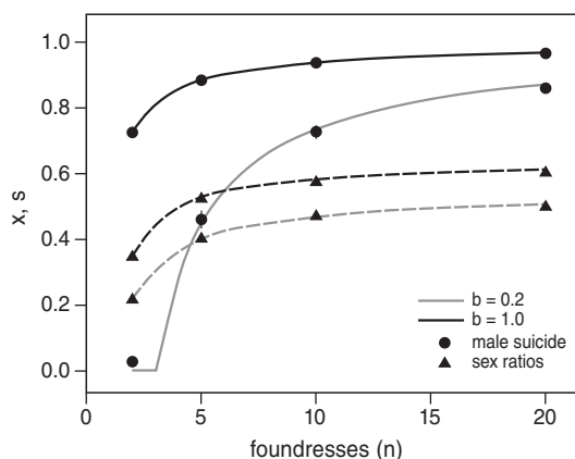
Figure 4.1 Male suicide can evolve and generate male biased equilibrium sex ratios. Equilibrium levels of male suicide rates x and brood sex ratios s (proportion male), as a function of number of females (foundresses, n ) per local patch. Solid curves represent male suicide as predicted by the analytical model for two values of b , the efficiency of recycling killed males into resources for sibs. Dashed curves represent co-evolved sex ratios as predicted by the analytical model. Note that male-biased sex ratios arise for some parameter combinations. The individual-based simulation results are presented by symbols representing averages \pm 1 standard deviation) of 10 replicates (circles: male survival; squares: sex ratios). The simulations fit the analytical predictions quite closely.
