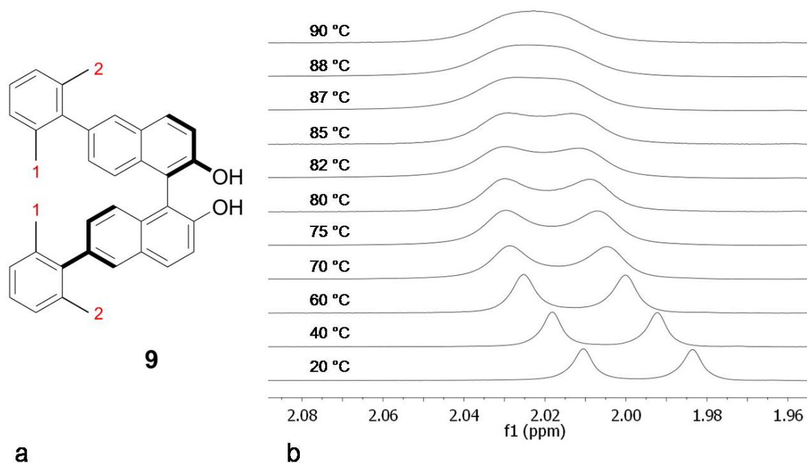
Figure 13. a: Structure of compound 9 with two different positions of methyl groups highlighted with numbers 1 and 2, b: The aliphatic part (1.96 – 2.08 ppm) of the ^1\text{H-NMR} spectra of 9 in anhydrous \text{DMSO-}d_6 at different temperatures.
