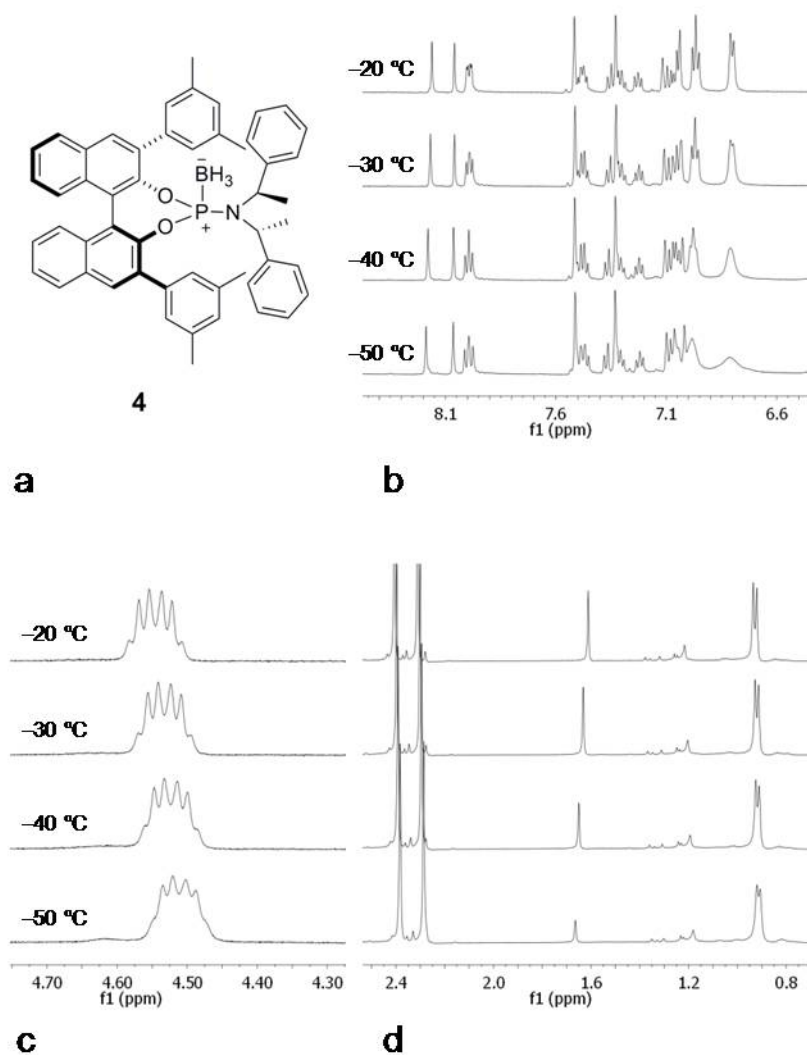
Figure 11. a: Structure of compound 4 , b: The aromatic part of the ^1\text{H-NMR} spectra of 4 in \text{CD}_2\text{Cl}_2 , c: The aliphatic part (4.30 – 4.70 ppm) of the ^1\text{H-NMR} spectra of 4 in \text{CD}_2\text{Cl}_2 , d: The aliphatic part (0.80 – 2.40 ppm) of the ^1\text{H-NMR} spectra of 4 in \text{CD}_2\text{Cl}_2 . The spectra are taken at different temperatures.
